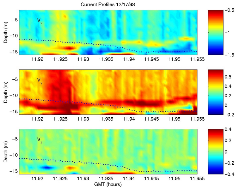
1d. Cross-shelf, along shore and vertical components of currents in the water column on 12/17/98 as determined by the ADCP on board.
