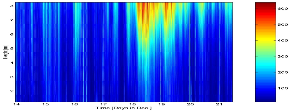
1e: TKE ((cm/s) 2 ) distribution in the water column over the 5-head ADCP during Dec 14 – 22, 1998 (Analysis by Matt Brennan).
