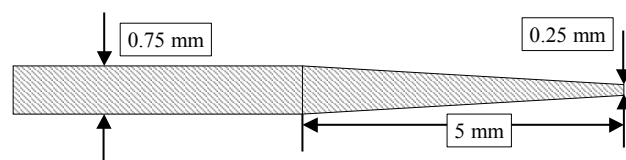
Figure 2. Illustration of the anode rod
