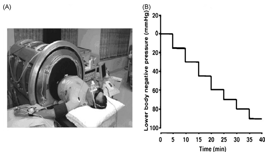
Fig. 1. Subject in the LBNP device (A) and the LBNP protocol (B).
