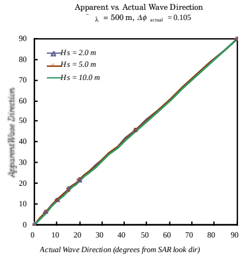
Figure 2: Apparent wave direction for \Delta\phi_{\text{Actual}} = 0.105 vs. actual wave direction with H_s = 2.0 m, 5 m and 10.0 m, and \lambda = 500 m.
