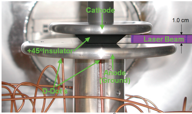
Figure 2. A close up photo a +45° insulator under test.
