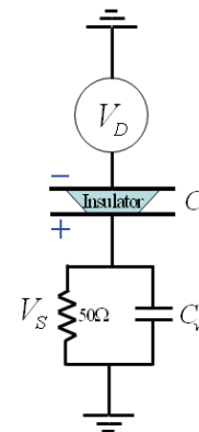
Figure 5: Lumped element circuit model of D-dot.
