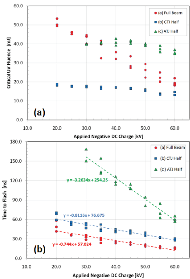
Figure10: (a) UV fluence data and (b) time to flash data for Full-beam, cathode-half and anode-half UV Illumination .
