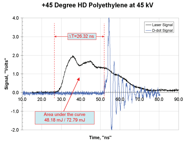
Figure 6. D-dot signal during flashover with laser power signal.
