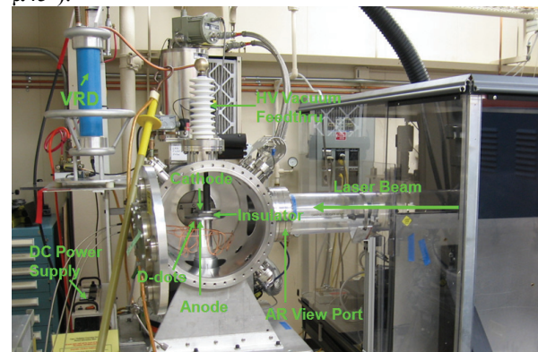
Figure 1. A photo of the UV-Insulator Testbed.
