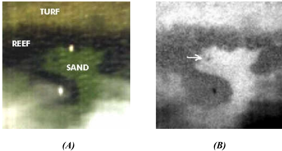
Figure 4. Pseudocolor PHILLS image (A) and band-math classified image (B) of the Horseshoe Reef area.
