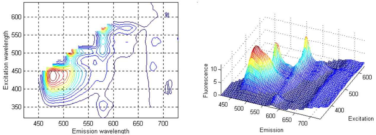
Figure 2. 3D excitation/emission spectrum for a specimen of the coral Montastraea cavernosa . Contour plot (left) and 3D surface plot.
