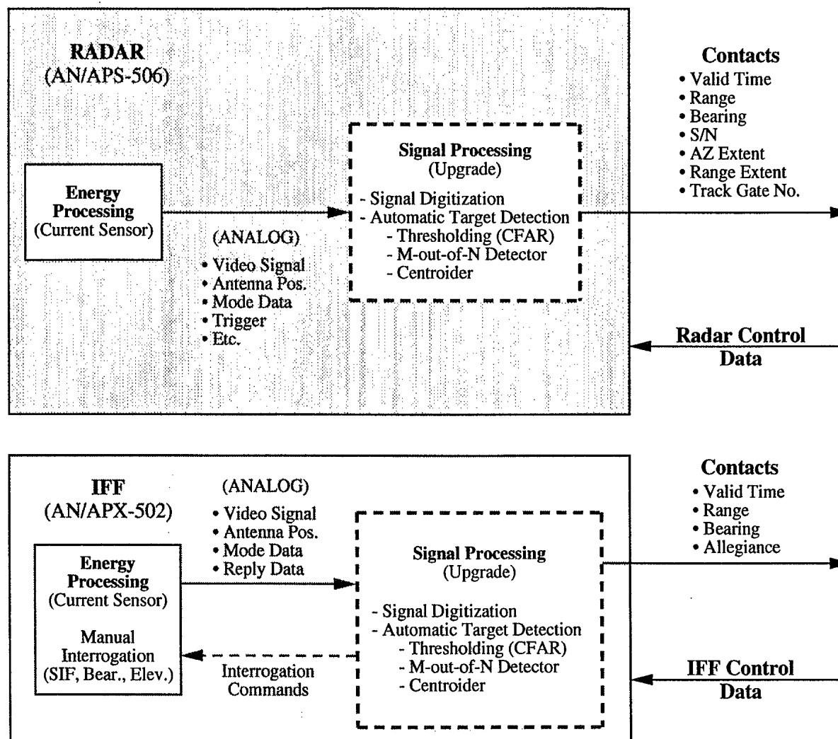
FIGURE 11 - Radar and IFF initial upgrades required for step 1
