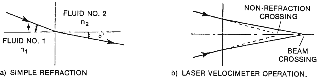
FIGURE 1. REFRACTION OF LIGHT BEAMS.
