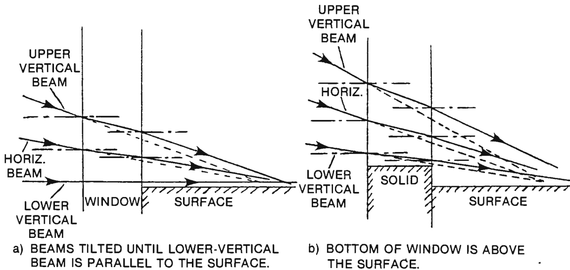
FIGURE 3. TILTED BEAM LASER VELOCIMETER OPERATION.
