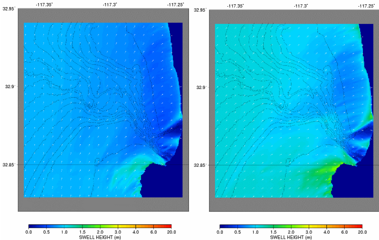
Figure 4: SWAN analysis of swell in the NCEX area for Sep 26, 2003 (nowcast) (left image) and Sep 29, 2003 (72 hours) (right image)
