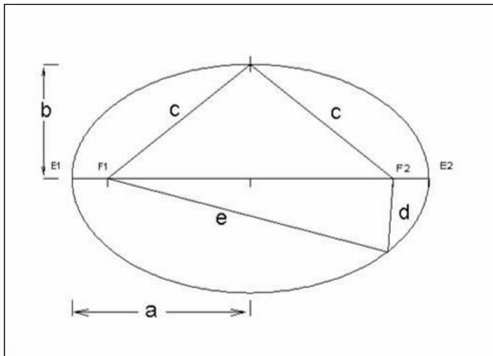
Figure 6-36. Sketch of ellipse associated with path length difference.
