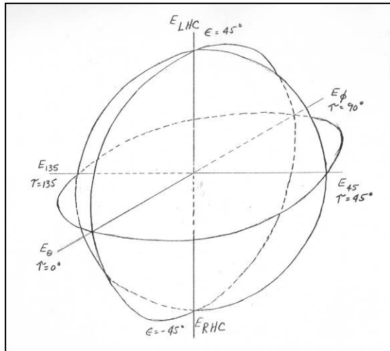
Figure 5-24. Poincare sphere definitions.
