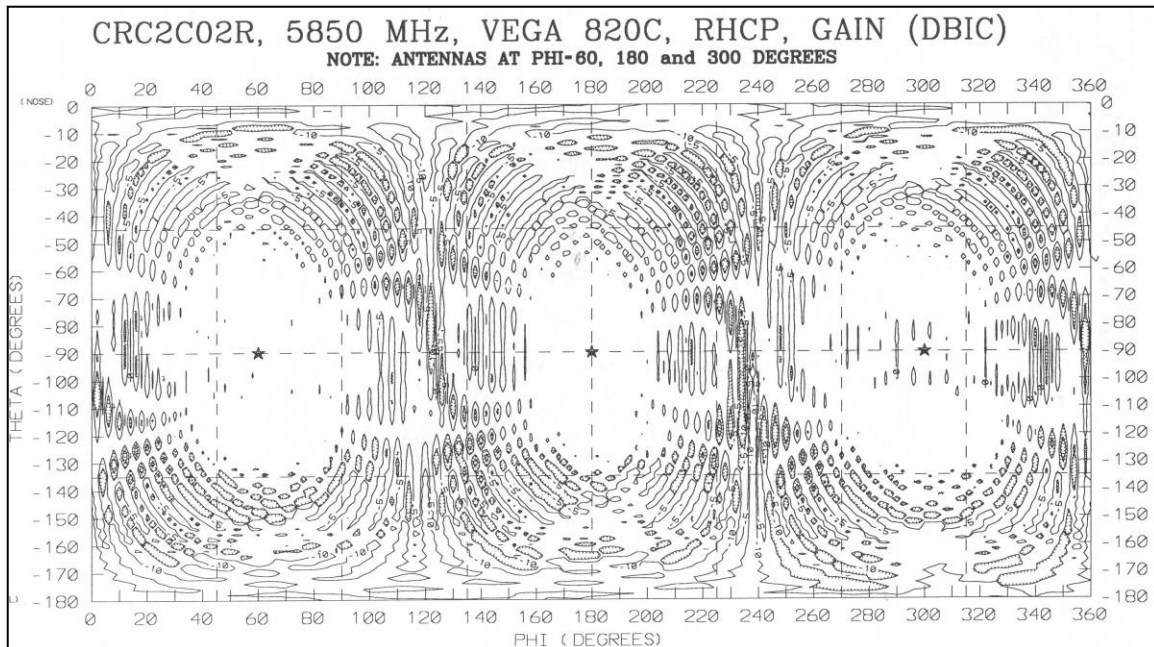
Figure 5-7. Contour plot of right hand circular gain for three vega antennas.
