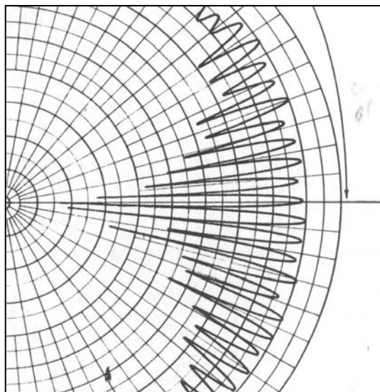
Figure 6-8. Analog pattern.
