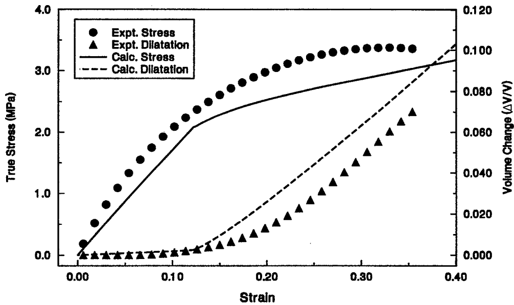
FIGURE 34 – Predicted mechanical behavior for treated glass bead/polyurethane composite based on best-guess parameters, c_o^t = 0.4
