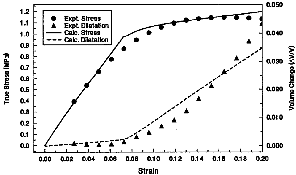
FIGURE C13 – True stress and dilatation behavior for composite N5FS
