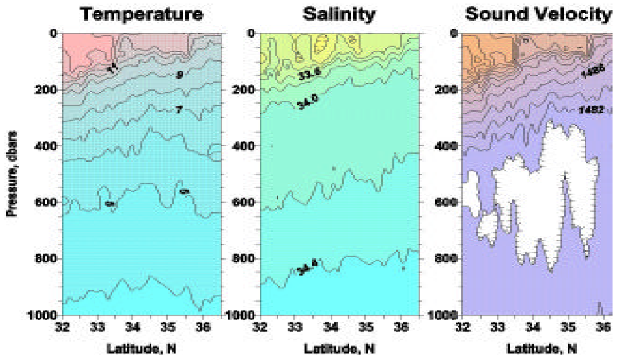
Figure 1. Surveyed temperature, salinity and sound speed sections between Hoke Seamount (~32° 06' N, 126° 54' W) and Pt Sur (~36° 18' N, 122° 23' W). The hydrographic data shows that isovels and isohalines above 400 m shoaled to the north. Below 400 m, the 6-7°C isotherms were shallowest at about 34.5°N, and deepened northward and was associated with poleward flow at intermediate depths. In the upper 100 m, two strong fronts were observed at 33.5°N and 36°N; the location of the former also coincided with the lens of low salinity surface water (S<33) associated with the core of southward flowing Subarctic water in the California Current. The deep sound channel had speeds less than 1480 m/s and was centered between 450 and 600 dbars.
