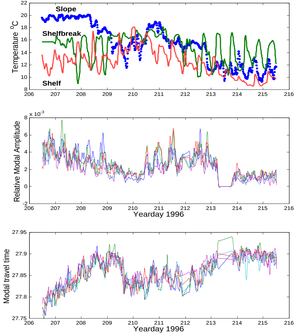
Figure 2. Measured thermocline temperature variability on the slope, shelfbreak and shelf (upper panel), and measured amplitude fluctuations (middle panel) and travel time fluctuations (lower panel) of the lowest five modes at 400 Hz.
