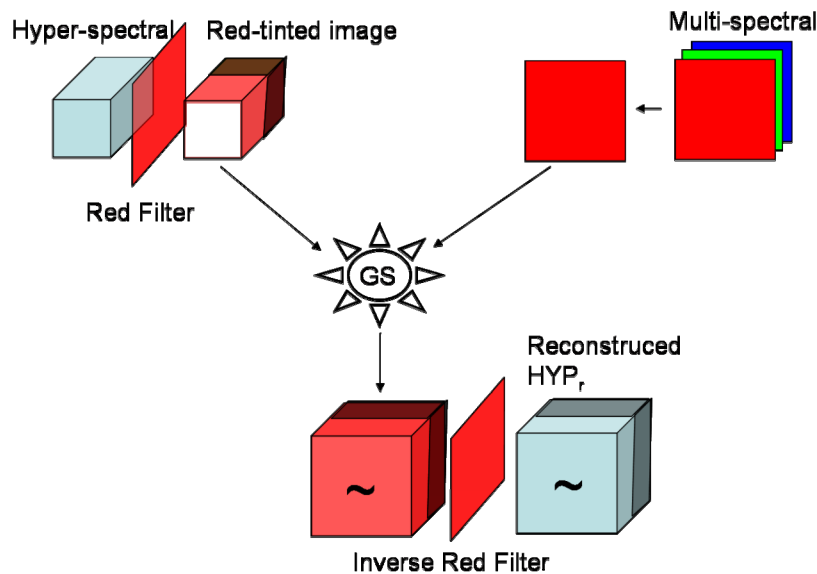
Figure 2. In the modified Gram-Schmidt approach each RGB channel is used only with the overlapping bands in the HSI image cube.
