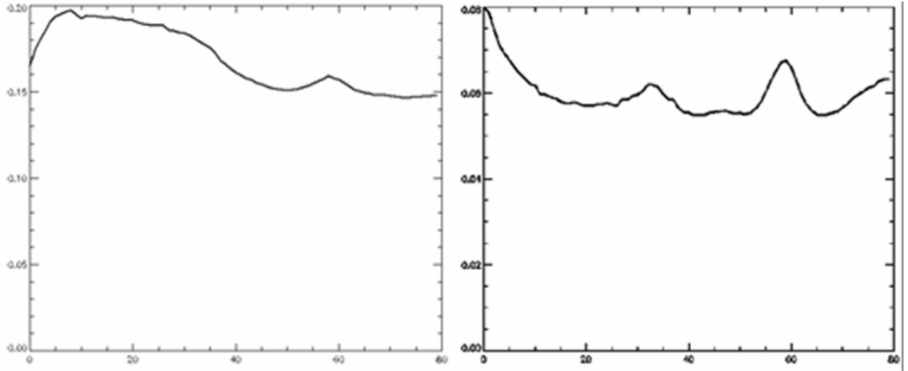
Figure 3. The graph on the left shows the errors between in the ideal case use the traditional Gram-Schmidt approach, range is ~15-20% over the spectrum. In the modified Gram-Schmidt approach (right graph) there is a marked reduction in the reconstruction error, range is ~6-8% over the spectrum.
