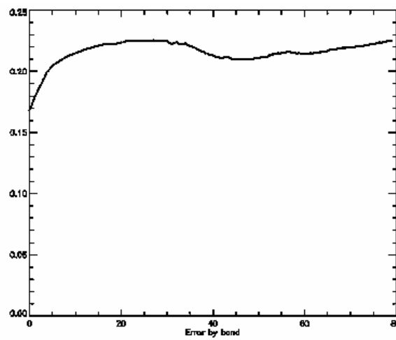
Figure 4. This graph shows the reconstruction error in the practical case, where the DSS imagery is used in the modified Gram-Schmidt approach to fusing the MSI/HSI data. The increase in the error range to ~22% results from differences in (1) the unknown calibration of the DSS, (2) view angle and its impacts on atmospheric and illumination contamination, and (3) pixel co-registration errors.
