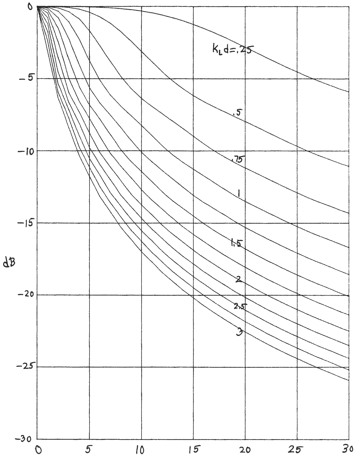
Figure 4. Degradation for k_0 d = \frac{\pi}{60} , \phi_\ell = \frac{\pi}{4} , \theta_\ell = \frac{\pi}{4}
