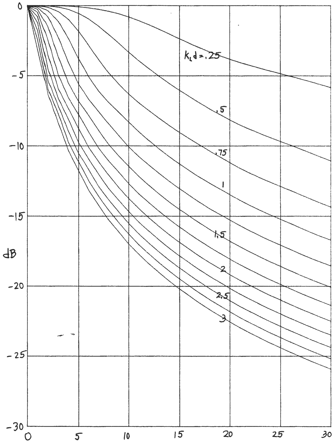
Figure 6. Degradation for k_0 d = \frac{\pi}{15} , \phi_0 = \frac{\pi}{4} , \theta_0 = \frac{\pi}{4}
