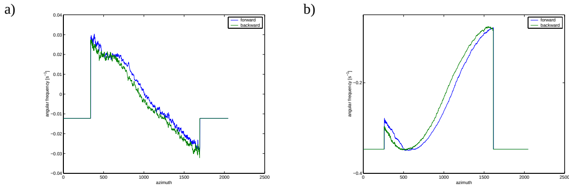
Figure 3: Illustration of the CHASP tracking algorithms for simulated moving object composed of five point targets in coloured noise with SCNR = 14 dB : a), Uniformly moving along track at 1 m/s; and b) Moving along track at 1 m/s with combined sway and heave circulation motion of 0.25 m amplitude with a period of 6.7 s.
