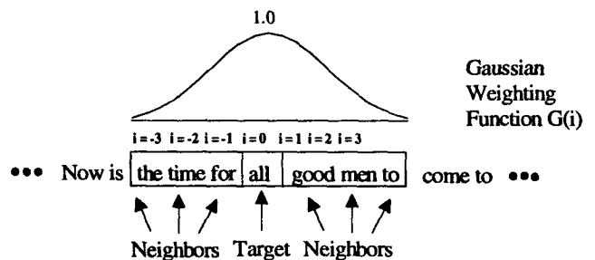
Figure 10. Original Bootstrap Window Calculation
