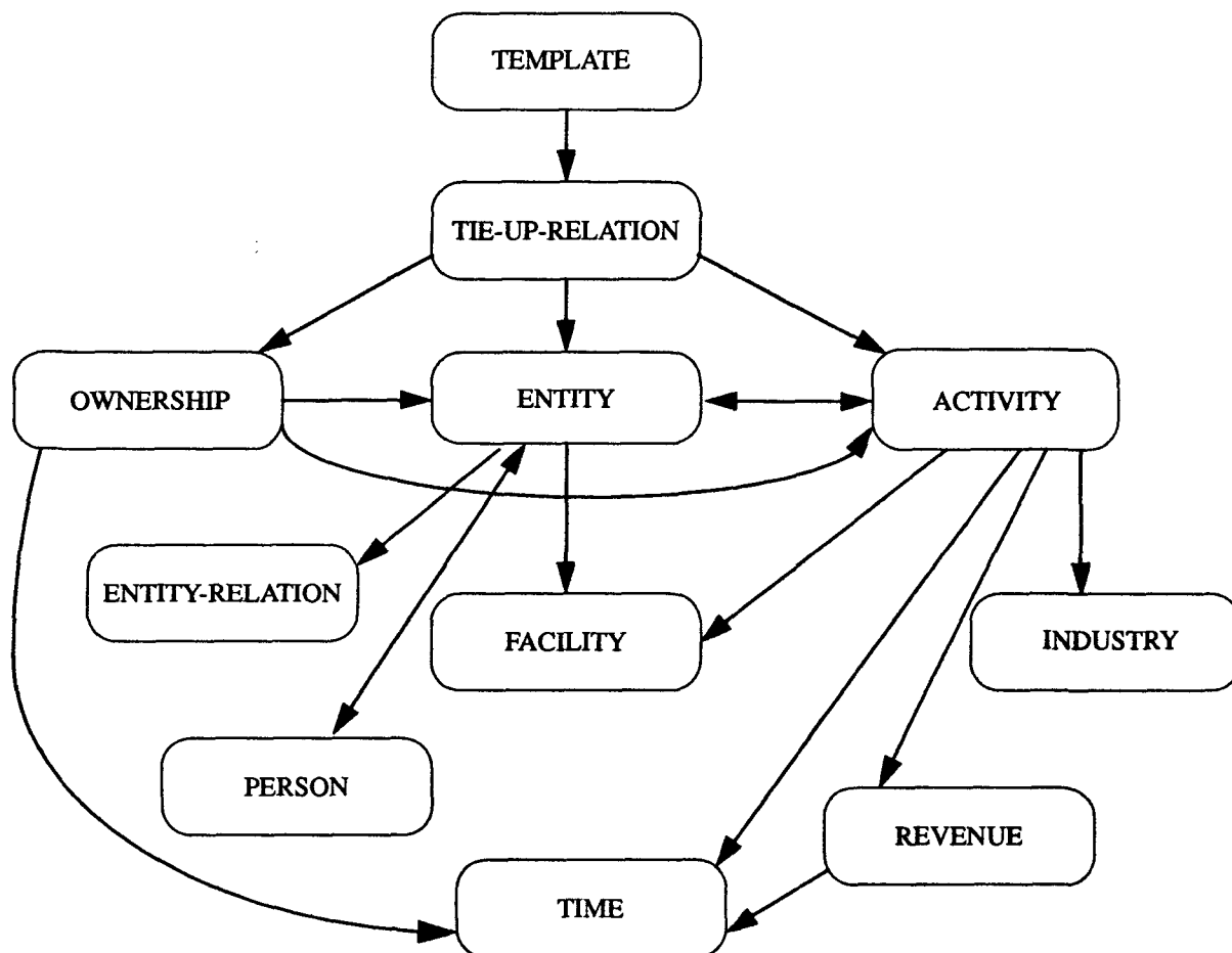
Figure 1: Joint Venture template object types (and pointers)
