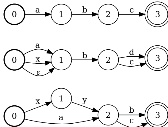
Figure 3.9: Three examples of word lattices: (a) sentence, (b) confusion network, and (c) non-linear word lattice.
