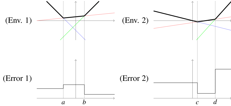
Figure 3.7: Each segment from the upper envelope (above) corresponds to a hypothesis with a particular error score, forming a piecewise constant error surface (below). The points a , b , c , and d are the transition points.
