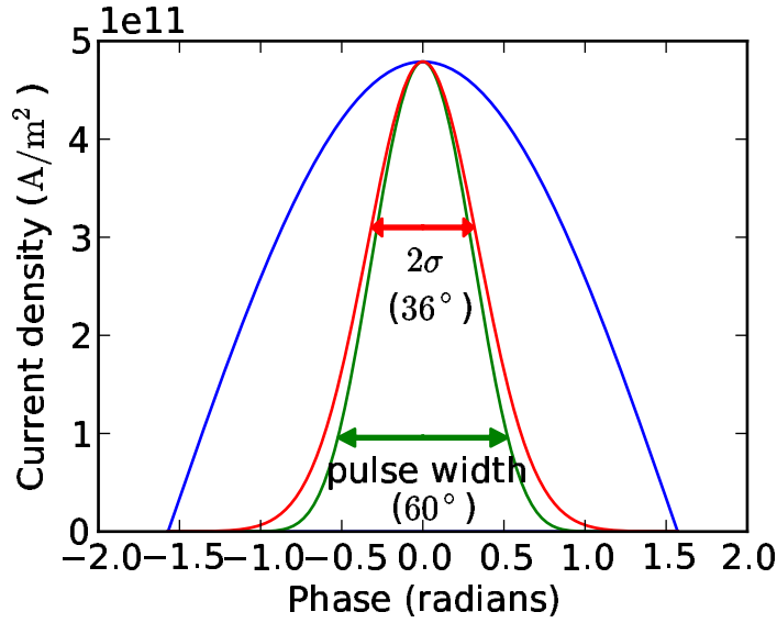
Figure 5.2: Pulse shape of electrons emitted from a field emission cathode in an RF field. The blue curve represents the RF field. The green curve is the current density as calculated using the approximate, one dimensional Fowler-Nordheim theory, where the green arrow shows the pulse width as defined above in the text. The red curve is the Gaussian approximation, where the red arrow shows the range covering one standard deviation to each side of the center.
