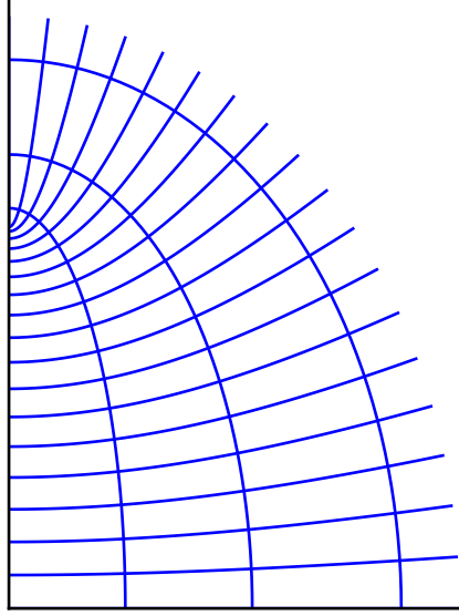
Figure 2.5: Alternate parameterization for an elliptic coordinate system. The ellipses are lines of constant \chi ; the hyperbolas are lines of constant \theta . In particular, \theta = \arccos \xi is plotted every 5^\circ between 0^\circ (z axis) and 90^\circ (r axis). We will often plot data as a function of this variable.
