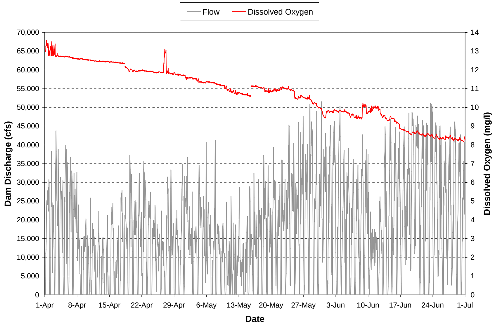
Plate 67. Hourly discharge and dissolved oxygen concentrations monitored in the “raw water supply line” at the Oahe powerhouse during the period April through June 2006. (Note: Gaps in dissolved oxygen plot are periods when the monitoring equipment was not operational.)
