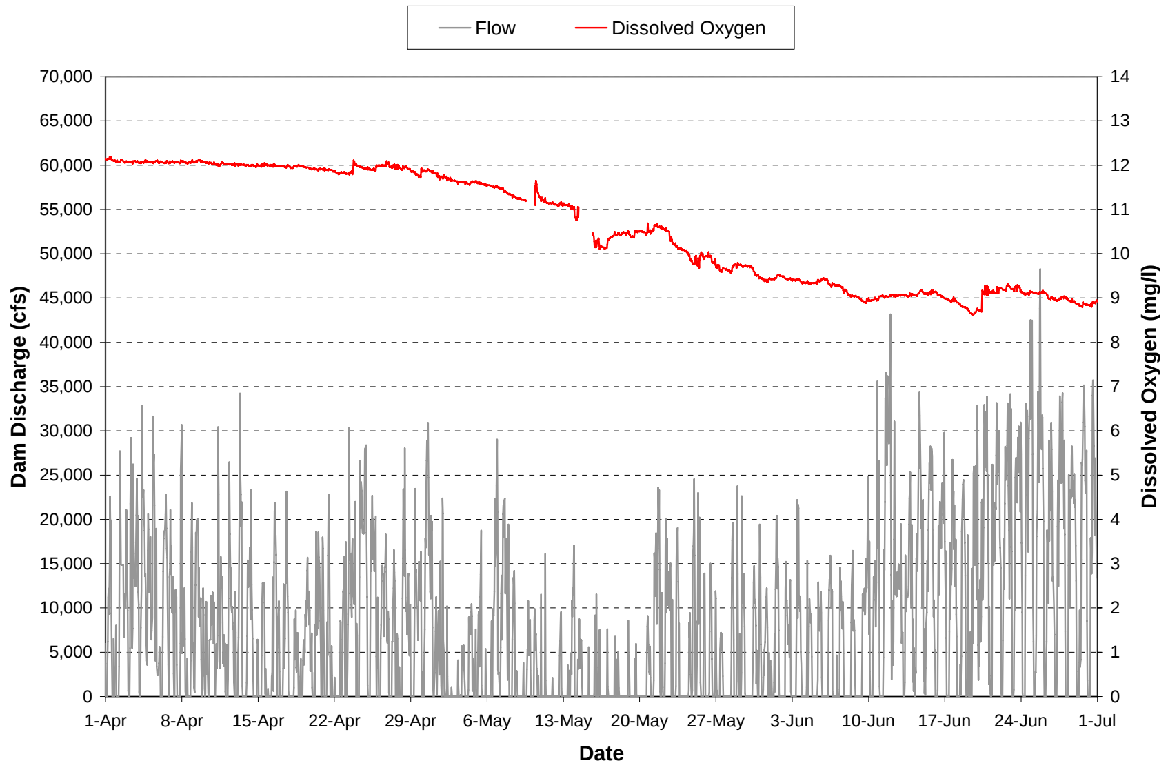
Plate 71. Hourly discharge and dissolved oxygen concentrations monitored in the “raw water supply line” at the Oahe powerhouse during the period April through June 2007. (Note: Gaps in dissolved oxygen plot are periods when the monitoring equipment was not operational.)
