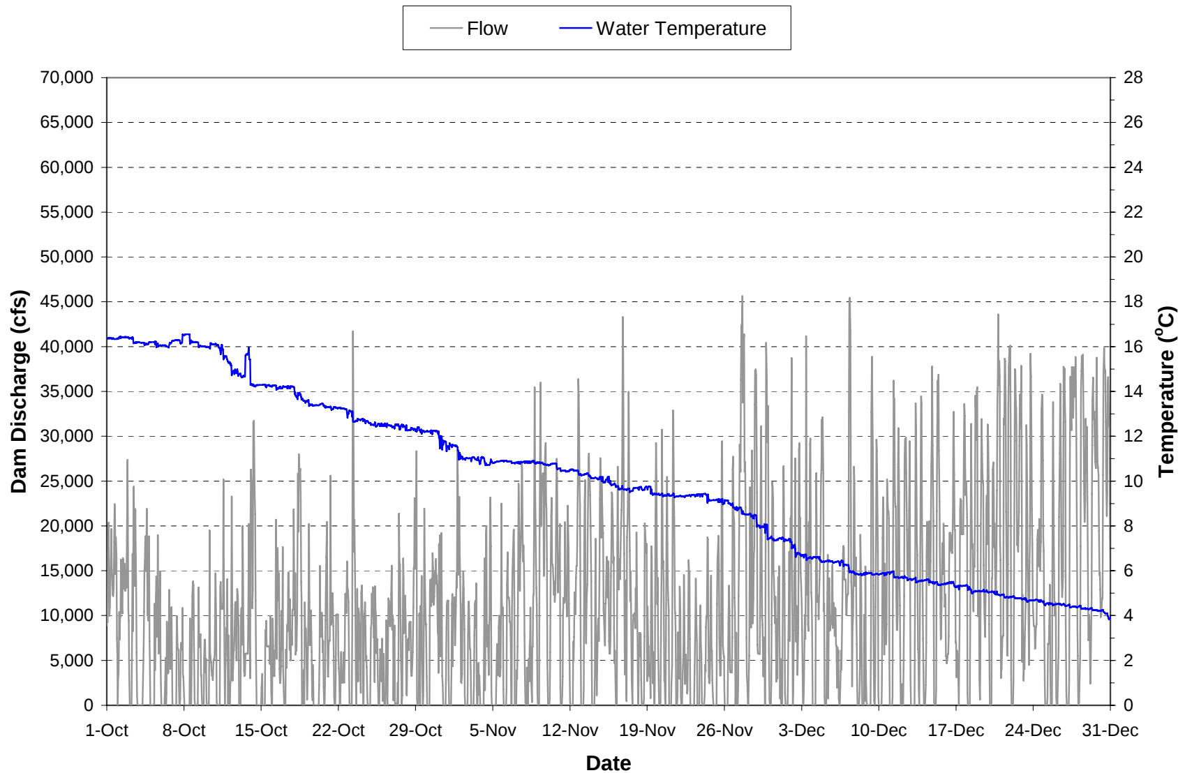
Plate 61. Hourly discharge and water temperature monitored in the “raw water supply line” at the Oahe powerhouse during the period October through December 2006.
