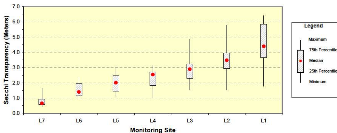
Figure 5.1. Box plot of Secchi transparencies measured in Oahe Reservoir at sites L1 through L7 during the 3-year period 2005 through 2007. (Note: monitoring sites are oriented on the x-axis in an upstream to downstream direction.)
