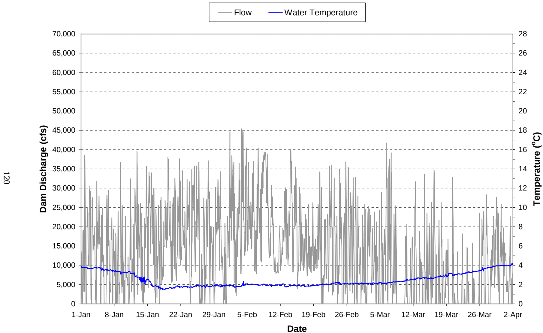
Plate 62. Hourly discharge and water temperature monitored in the “raw water supply line” at the Oahe powerhouse during the period January through March 2007.
