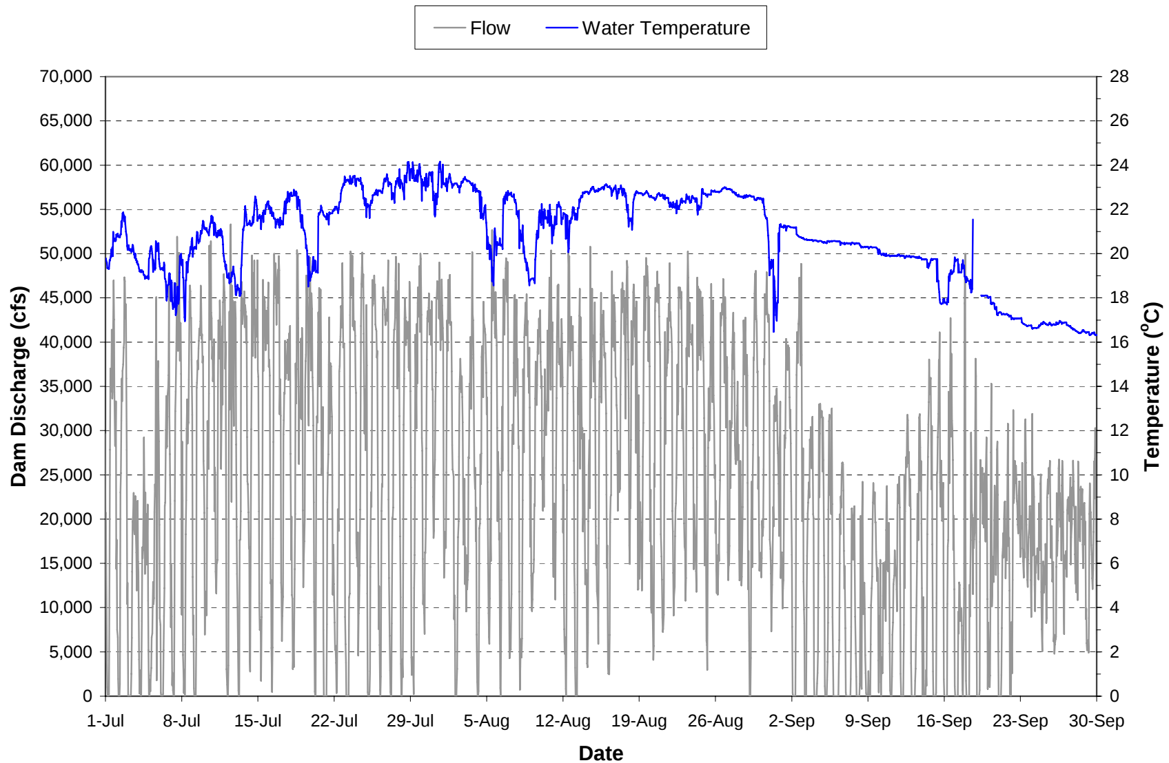
Plate 60. Hourly discharge and water temperature monitored in the “raw water supply line” at the Oahe powerhouse during the period July through September 2006.
