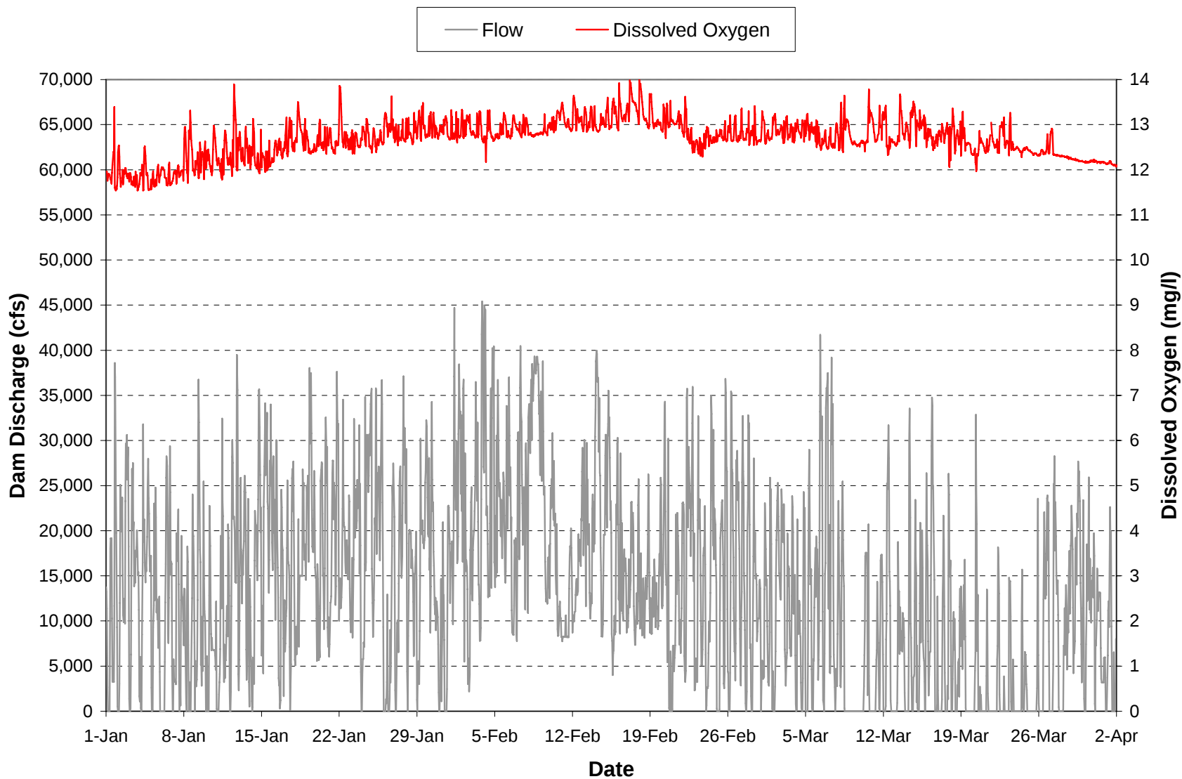
Plate 70. Hourly discharge and dissolved oxygen concentrations monitored in the “raw water supply line” at the Oahe powerhouse during the period January through March 2007. (Note: Gaps in dissolved oxygen plot are periods when the monitoring equipment was not operational.)
