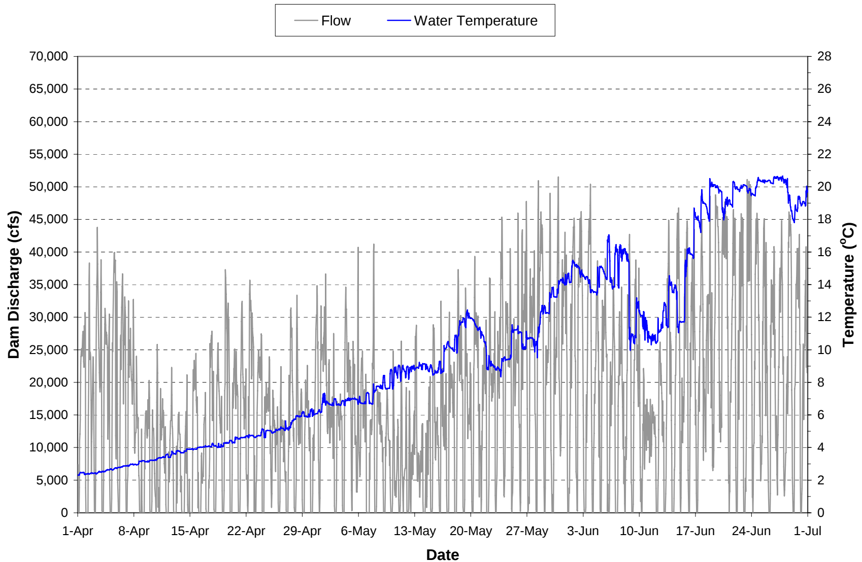
Plate 59. Hourly discharge and water temperature monitored in the “raw water supply line” at the Oahe powerhouse during the period April through June 2006.
