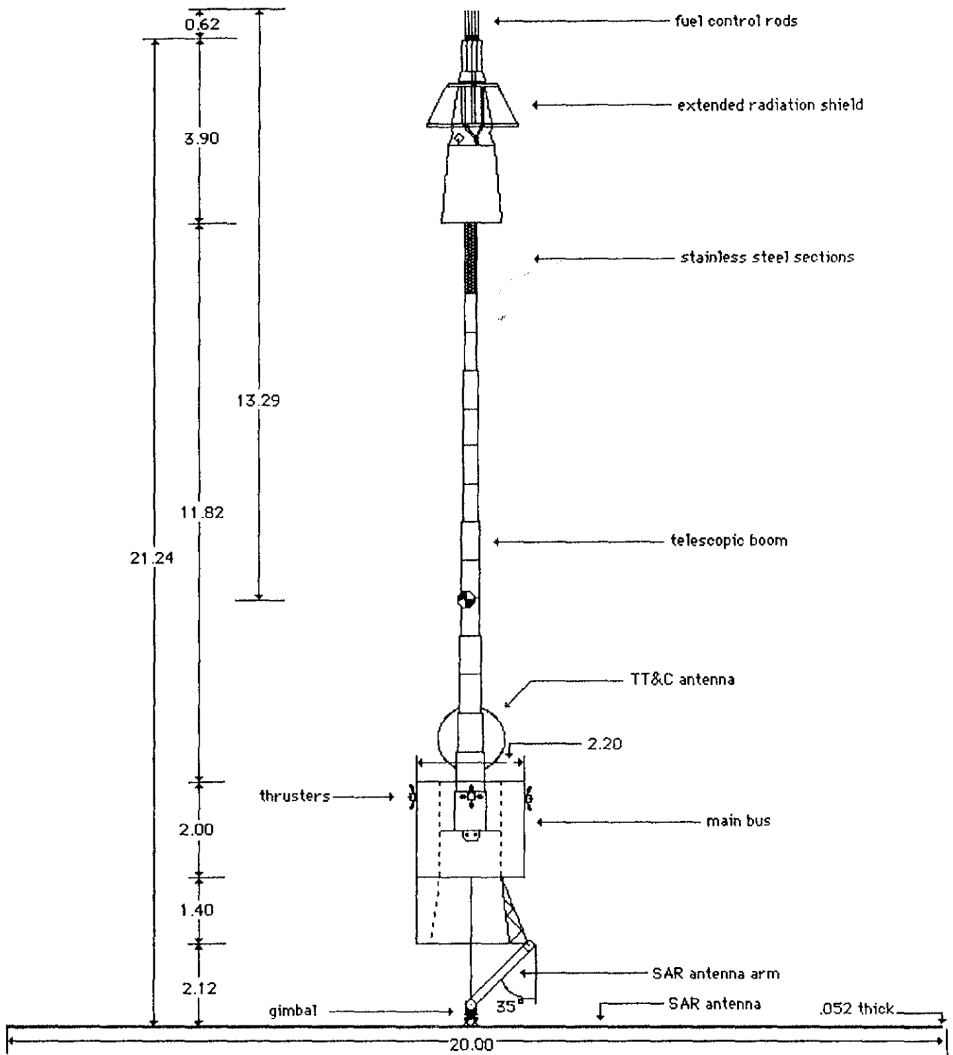
Figure 4. Side View.
