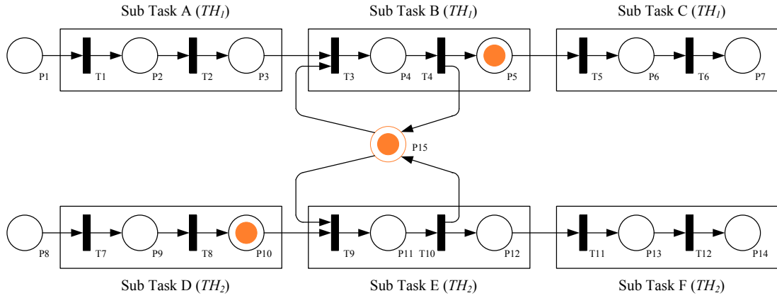
Figure 18: Petri-Net common resource use coordination (Event n + 2 )
