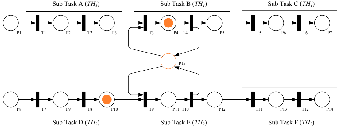
Figure 17: Petri-Net common resource use coordination (Event n + 1 )
