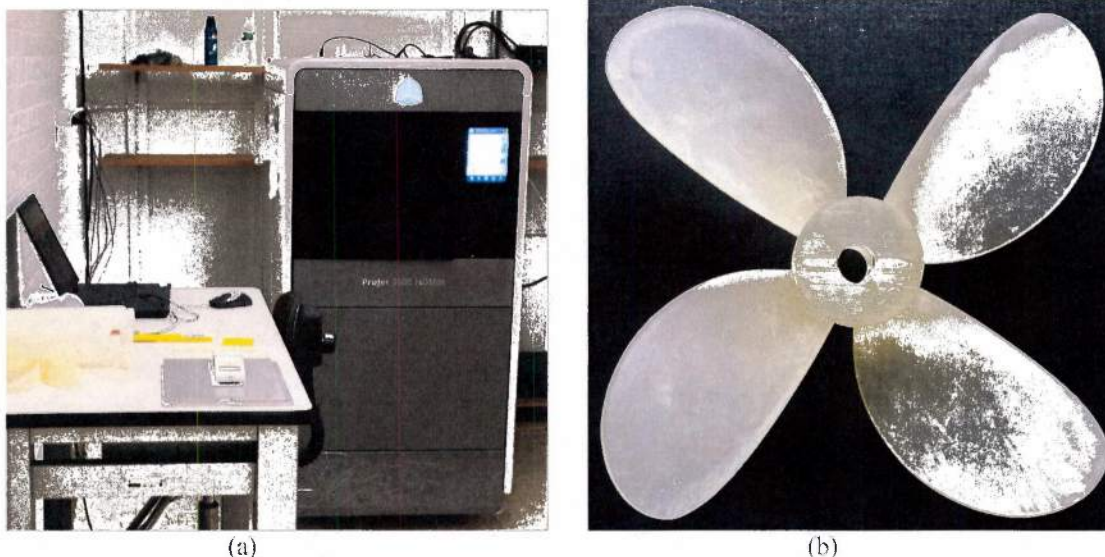
Figure 12: (a): ProJet 350 HD Max, (b): Eight inch 3D printed propeller.
