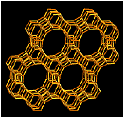
Zeolite AFI - Tetrapropylammonium Fluoride AIPO-5
