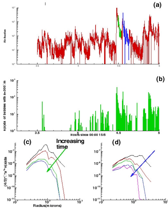
2: (a) Time series measurements of air fraction measured in the surf. A large double peak occurs due to enhanced breaking. (b) Concentration of bubbles of radius 300 microns, resonant at a frequency of 12 kHz corresponding to our propagation path. (c,d) Bubble size evolution following wave breaking. The two sets of curves correspond to the periods shown as green and blue respectively in (a).
