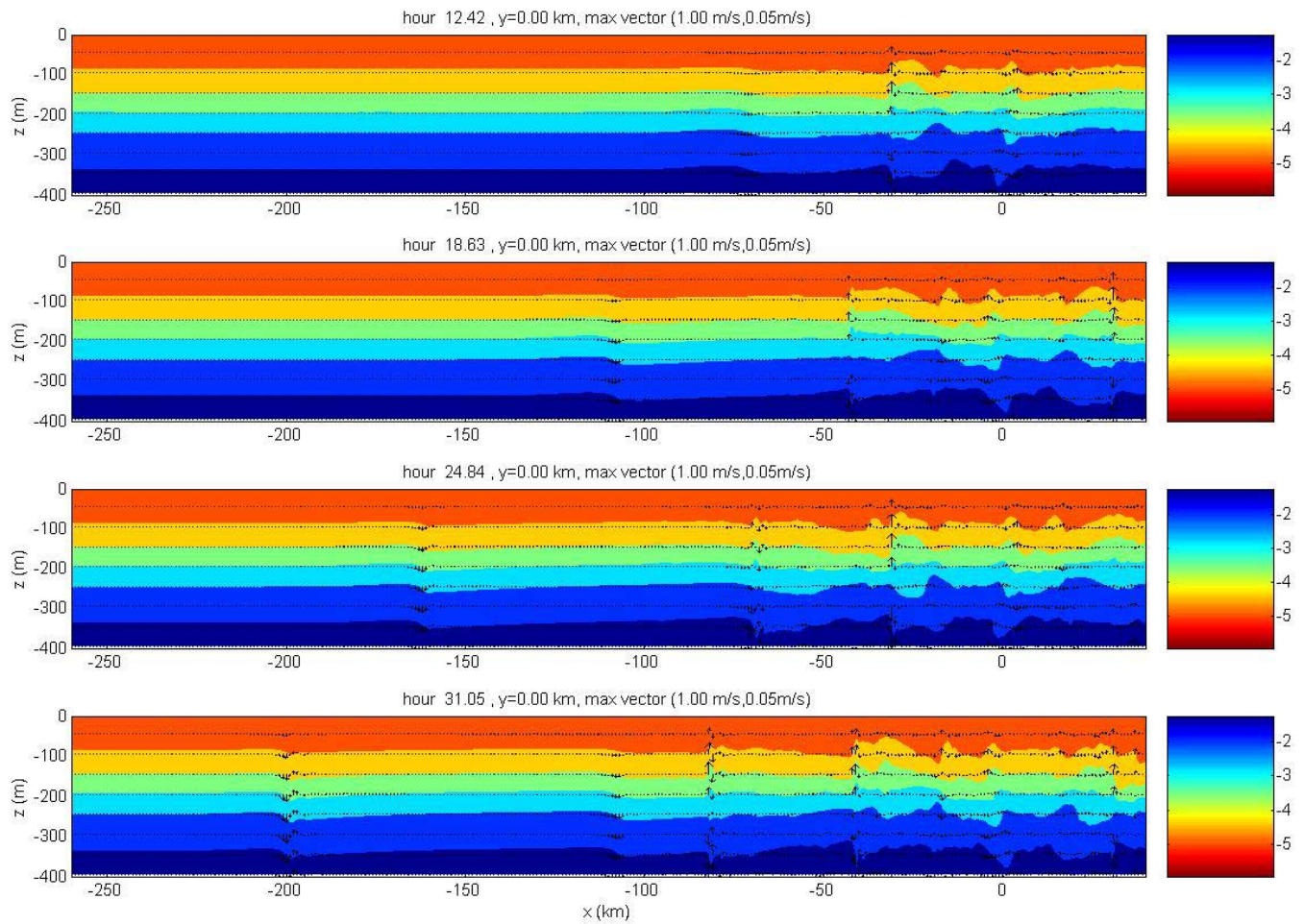
Figure 1: Evolution of the internal tide into a tidal bore and rank-ordered solitary waves. Contours represent perturbation density in kg/m 3 . Waves are generated by the barotropic tides over a ridge at x = 0 km.
