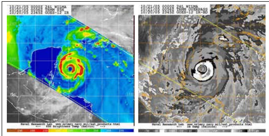
Figure 1. Coincident Hurricane Wilma IR Dvorak enhancement (right panel) and TMI 85 GHz H-pol brightness temperatures ( T_b , left panel) near 0000 GMT 21 October, 2005 illustrating inability of IR data to view double eyewalls clearly seen with passive microwave data. Grid lines are 2 deg x 2 deg.
