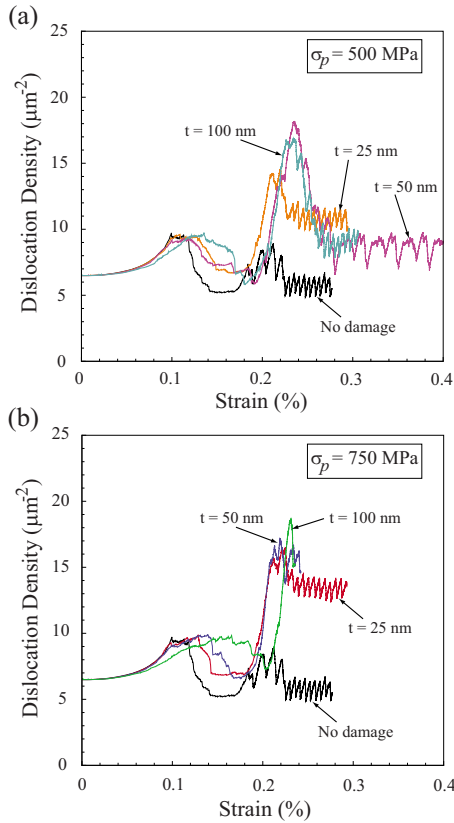
FIG. 2. (Color online) Dislocation density versus strain for a D=0.75\ \mu\text{m} micropillar having two precipitate strengths: (a) \sigma_p=500\ \text{MPa} and (b) \sigma_p=750\ \text{MPa} . Both cases produce an initial increase in dislocation density, however this density persists into the steady-state regime for the larger precipitate strength.
