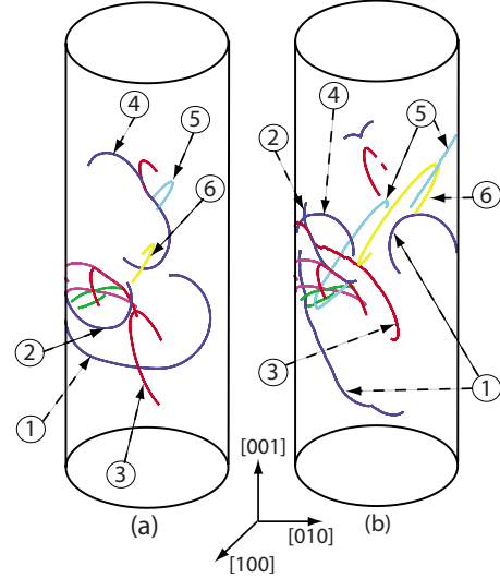
FIG. 1. (Color online) Microstructure of a D=0.75\text{ }\mu\text{m} micropillar at 0.17% strain. (a) No damage layer. (b) Damage layer depth t=100\text{ nm} and precipitate strength of \sigma_p=750\text{ MPa} is used. The precipitates are not plotted for clarity. The numbers encircled reference the same dislocations in both simulations.
