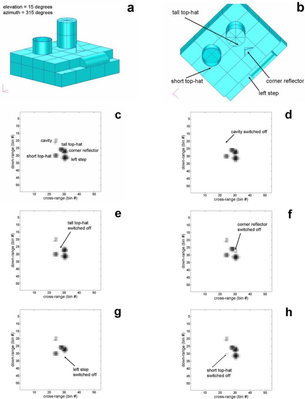
Figure 9 An illustration of contributions from various scattering primitives to the computed SAR images. a) visual view of SLICY as seen by the radar, b) corresponding view of the SAR image projection, c) scattering primitives on SLICY, d) to h) computed SAR images with a different scattering primitive switched off, one at a time.
