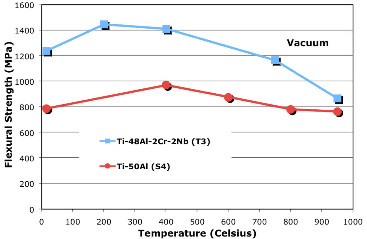
Figure 77: Comparison of flexural strength v. temperature between Ti-48Al-2Cr-2Nb (T3) and Ti-50Al (S4) alloy in vacuum.
