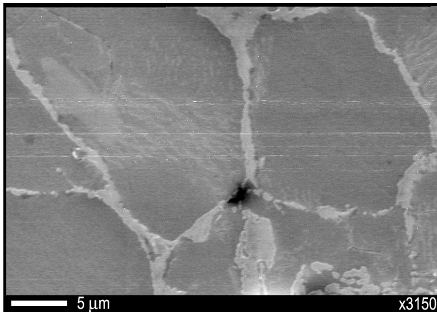
Figure 36: SEM of P2C consolidated sample S2 showing \alpha_2 (Ti 3 Al) phase segregated at the grain boundaries
