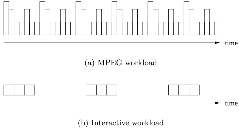
Figure 5.1: New generated workloads in Hourglass
