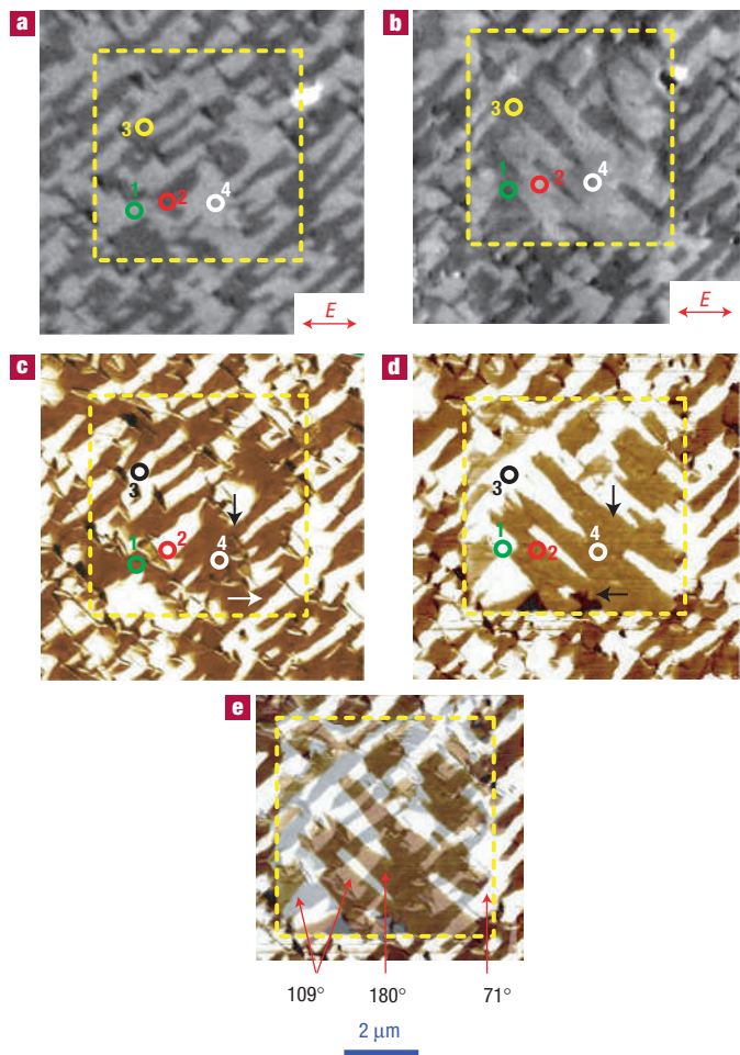
Figure 5 PEEM and in-plane PFM images of the same area of a BiFeO 3 film before and after electrical poling. a,b , PEEM images before ( a ) and after ( b ) poling. The arrows show the X-ray polarization direction during the measurements. c,d , In-plane PFM images before ( c ) and after ( d ) poling. The arrows show the direction of the in-plane component of ferroelectric polarization. Regions 1 and 2 (marked with green and red circles, respectively) correspond to 109° ferroelectric switching, whereas 3 (black and yellow circles) and 4 (white circles) correspond to 71° and 180° switching, respectively. In regions 1 and 2 the PEEM contrast reverses after electrical poling. e , A superposition of in-plane PFM scans shown in c and d used to identify the different switching mechanisms that appear with different colours and are labelled in the figure.
