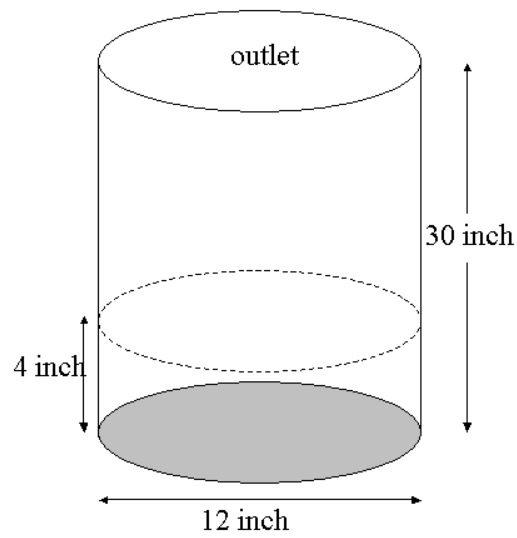
Figure 9. Geometry of the Actual Full Scale Reactor
