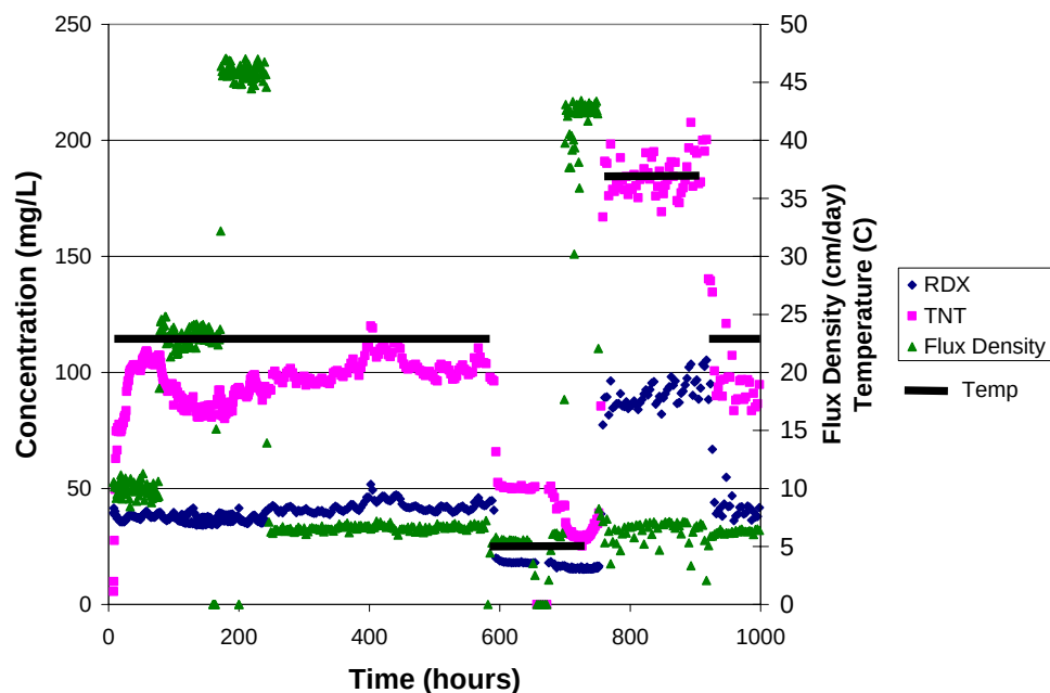
Figure 26. Test 1: Concentration and Flux Density
