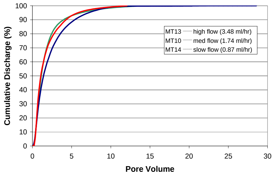
Figure 48. Effect of Flow – Cumulative Discharge, TNT
