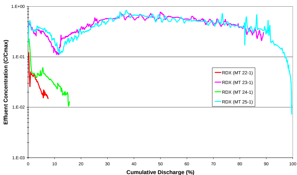
Figure 79. Effect of Energetic Material Particle Size – Cumulative Discharge, RDX
