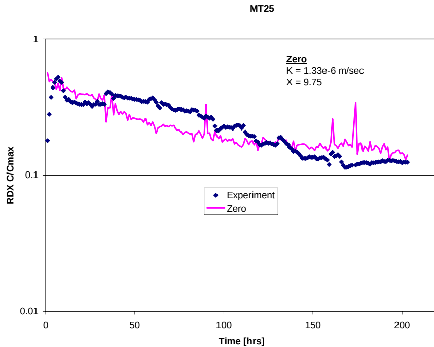
Figure A-17. Data-Model Comparison for MT25
