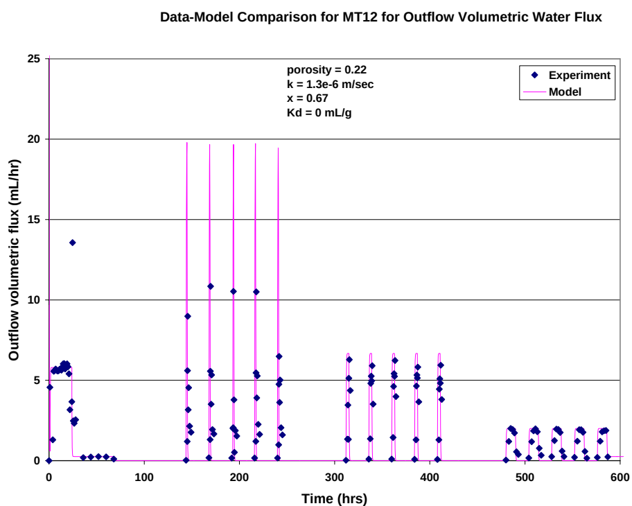
Figure 99. Data-Model Comparison for MT12 for Outflow Volumetric Water Flux
