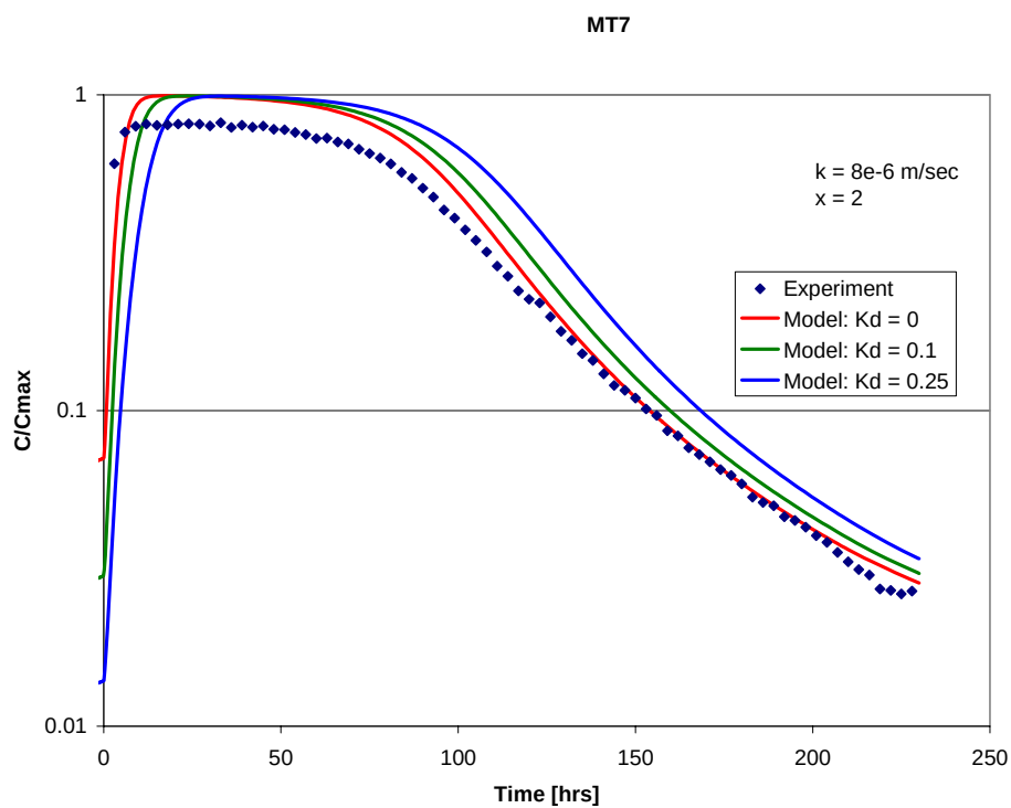
Figure 89. Effect of Solid Sorption Coefficient K_d on Model Response for MT7
