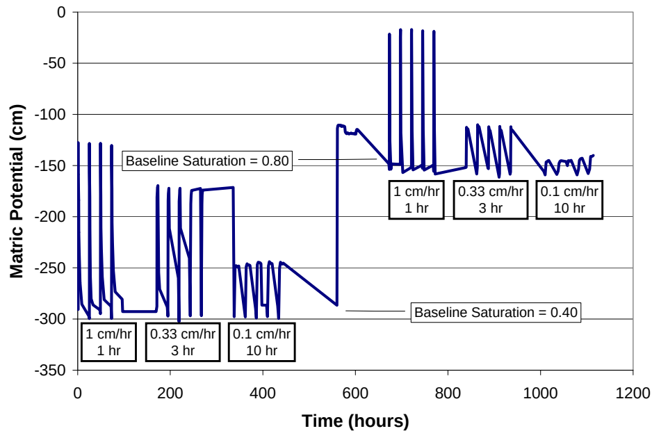
Figure 63. Column Matrix Potential (Tensiometer 1) During Pulse Test MT5
