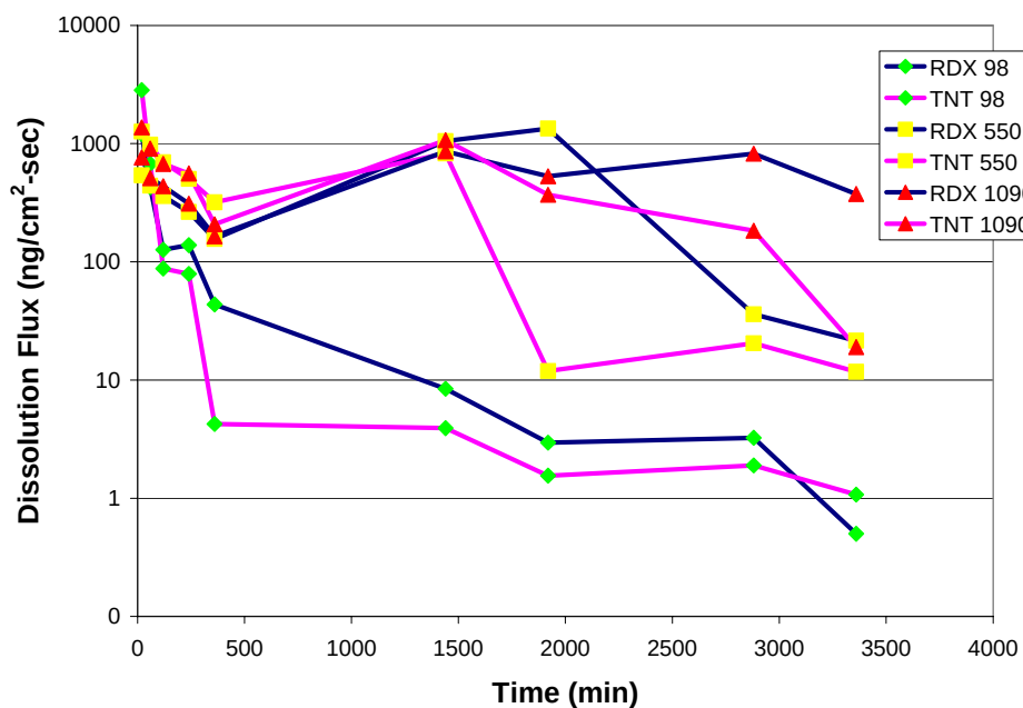
Figure 25. Derived Dissolution Flux for Comp B Particles in Water
