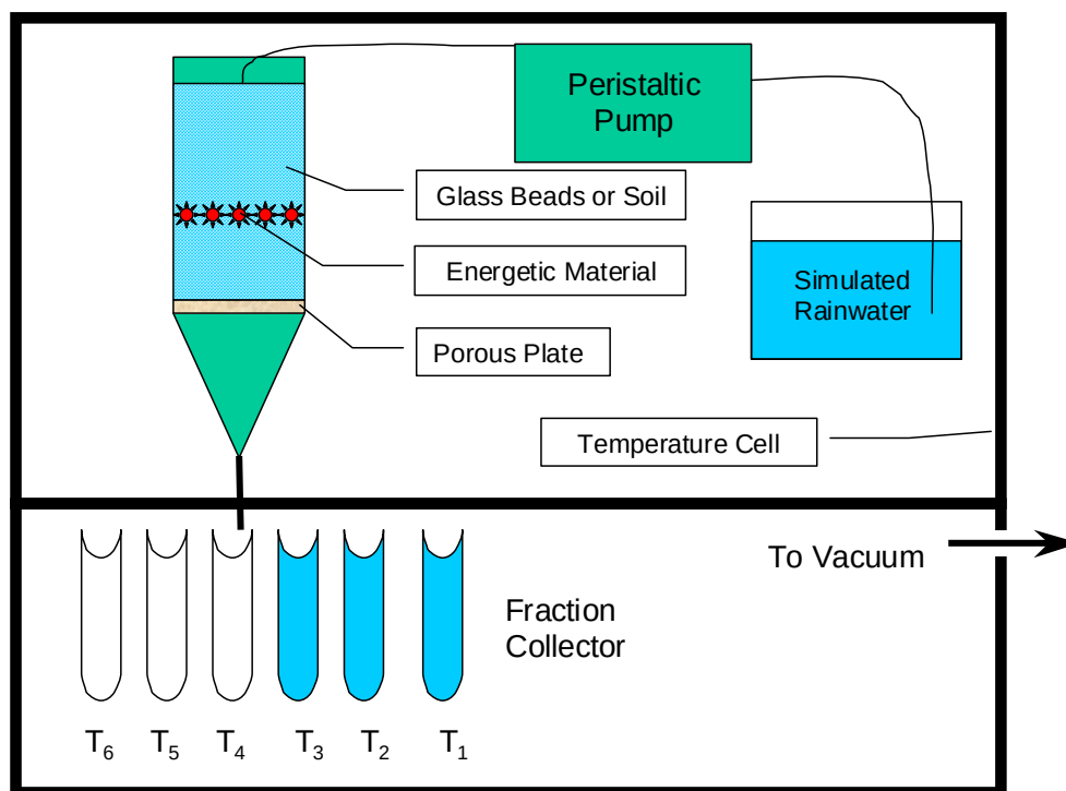
Figure 5. Laboratory Experimental Apparatus
