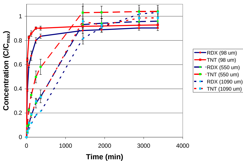
Figure 24. Full Duration Dissolution Results
