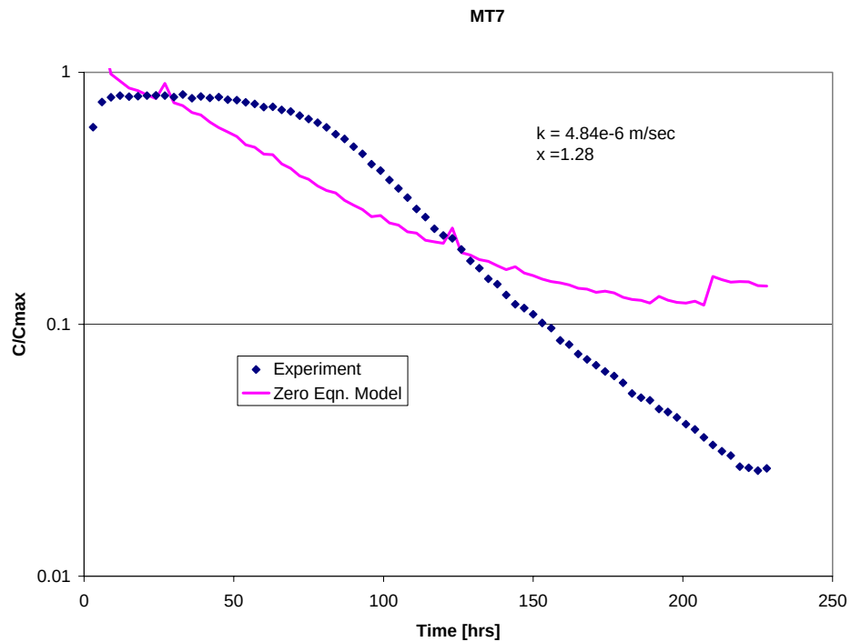
Figure A-2. Data-Model Comparison for MT7
