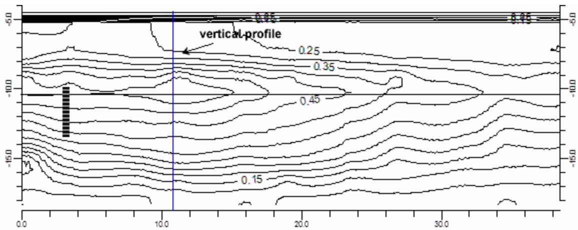
Figure 22. Differential resistivity profile for 3/24/05 (scales are in feet, the horizontal distance is relative to the upgradient electrode location, the vertical scale is depth below the surface).
