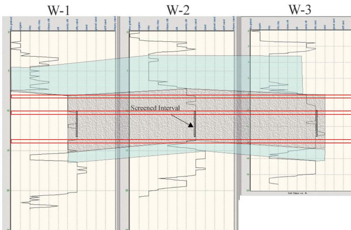
Figure 2. Test site stratigraphy based on preliminary SCAPS piezocone pushes. Also shown are the screen intervals of three monitoring wells that surround the test site and the depth intervals (in red) of the piezometer screens.
