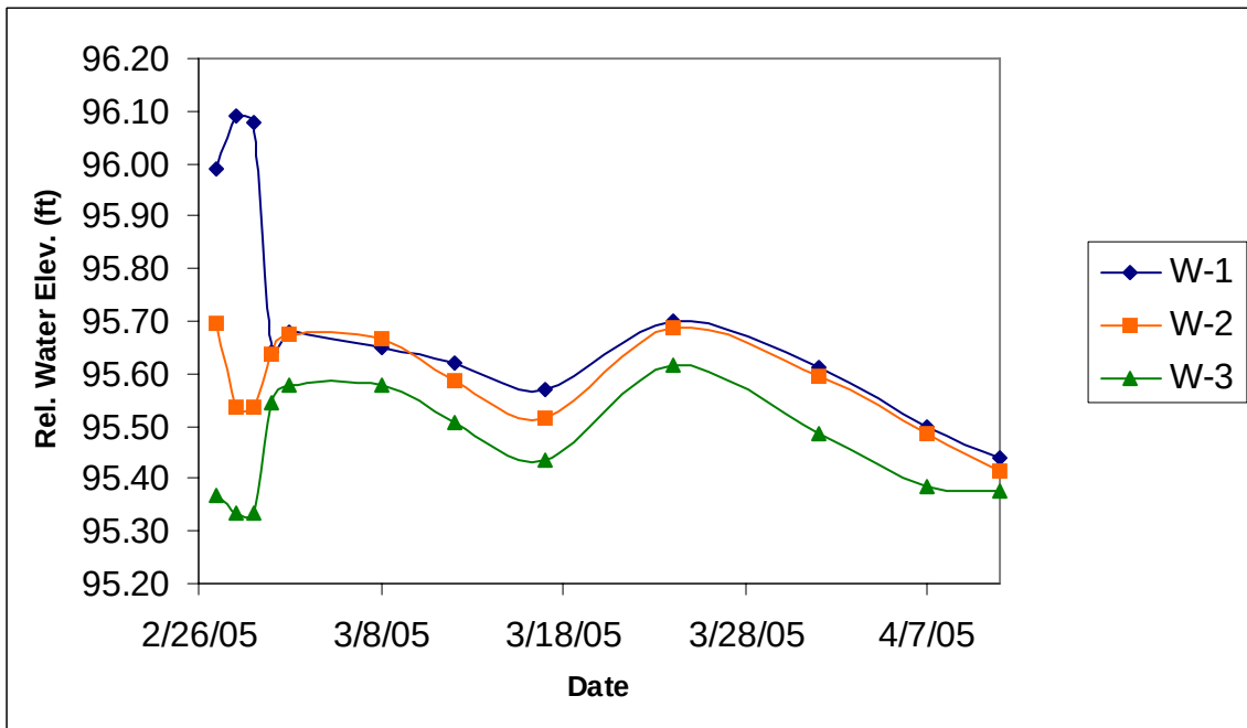
Figure 5. Relative water level elevations in perimeter wells.
