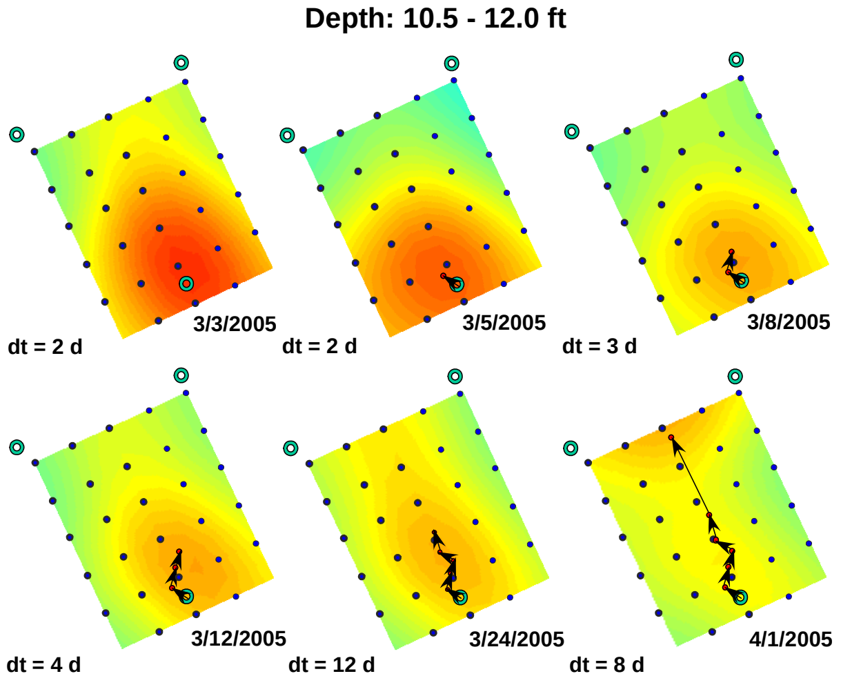
Figure 15. Contours of the differential electric resistivity in the upper zone of the silty sand formation ( z=10.5-12.0 ft) between the date of survey (marked for each contour) and February 28, 2005. The full scale of the color code (red to blue) is +2 to -2 Ohm-meter. Warm color means conductivity increases (resistivity decrease) and cool color means conductivity decreases and resistivity increases. The dt value refers to time in days between the mapped survey shown and the previous survey.
