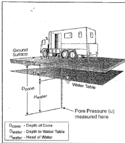
Figure 2-2. Estimates of Ground Water Table. Dissipated pore pressure at the depth of cone ( D_{cone} ) reflects head of water ( H_{water} ). The depth to water table ( D_{water} ) therefore equals D_{cone} minus H_{water} .
