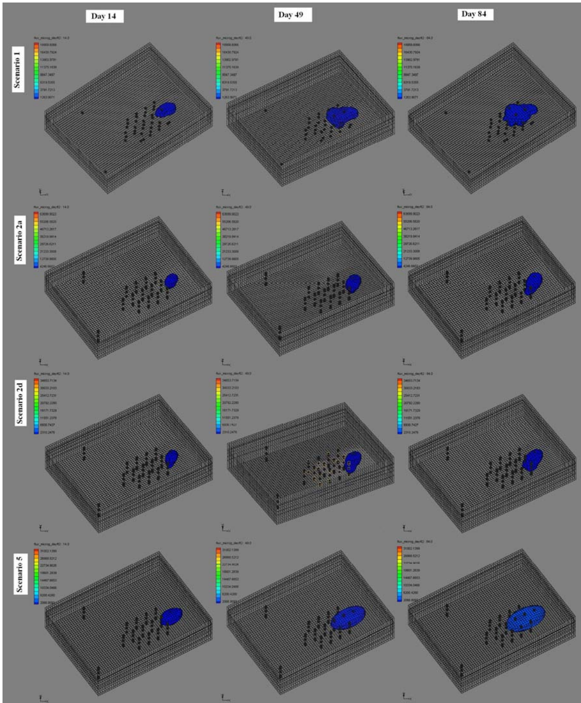
Figure 7. Isosurfaces showing a flux value of 30 µg/ft 2 /day, which represents a concentration of 35 ppb moving at the average groundwater velocity at the site (0.03 ft/day).
