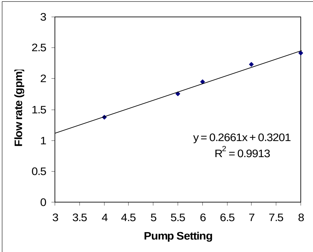
Figure 9. Pump calibration curve.
