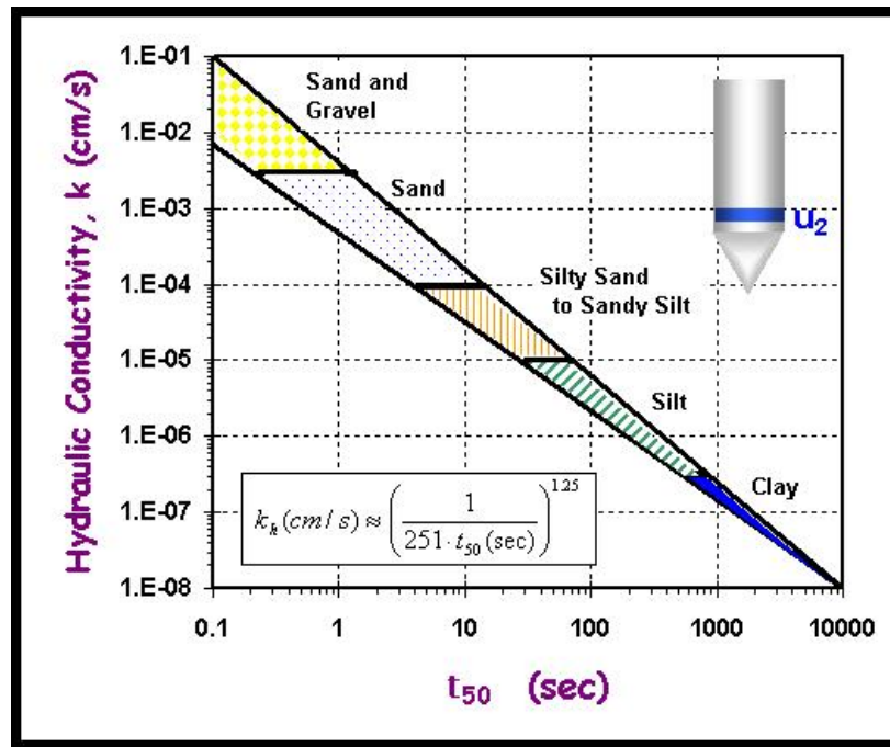
Figure 2-5. Parez and Fauriel (1988) Relationship Between K and t_{50} .
