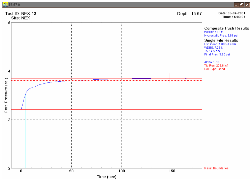
Figure 2-3. Pressure Dissipation Curve. The final pressure ( D_{cone} ), time for dissipation, and hydraulic conductivity can all be estimated using the dissipation curve.
