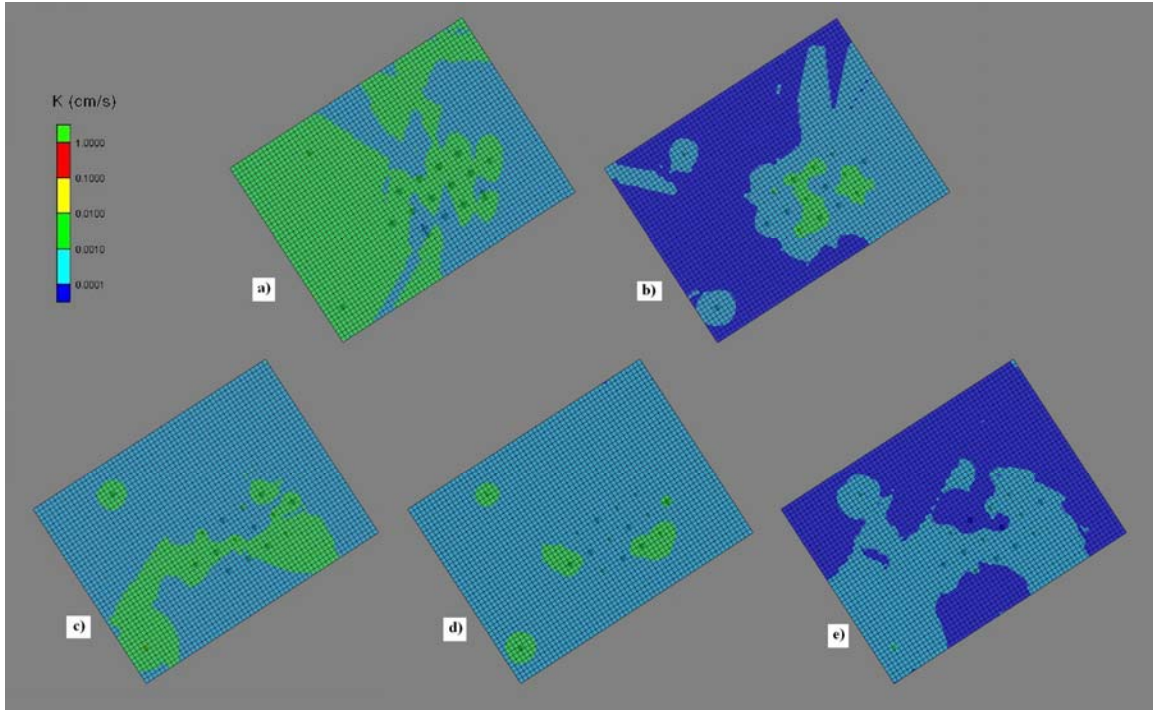
Figure 5. Hydraulic conductivity distributions for a) Kwell, b) Klookup, c) Kmax, d) Kmean, and e) Kmin. K values are in cm/s and each contour represents an order of magnitude change in K.
