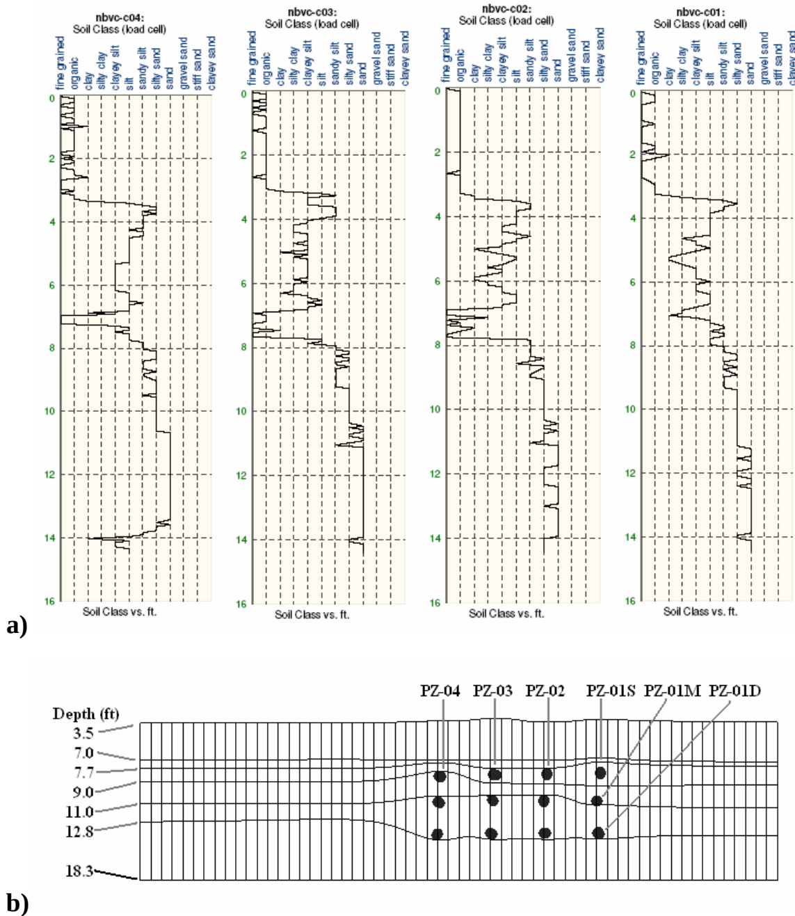
Figure 2. a) Stratigraphy inferred from SCAPS pushes for row 1 of piezometer cluster (PZ-01 – PZ-04). Vertical axis is depth below ground surface in feet. b) GMS grid showing layer boundaries for same vertical transect, showing location of screen centers for nested piezometers. Piezometers were denoted by number and depth (Shallow, Middle, and Deep).
