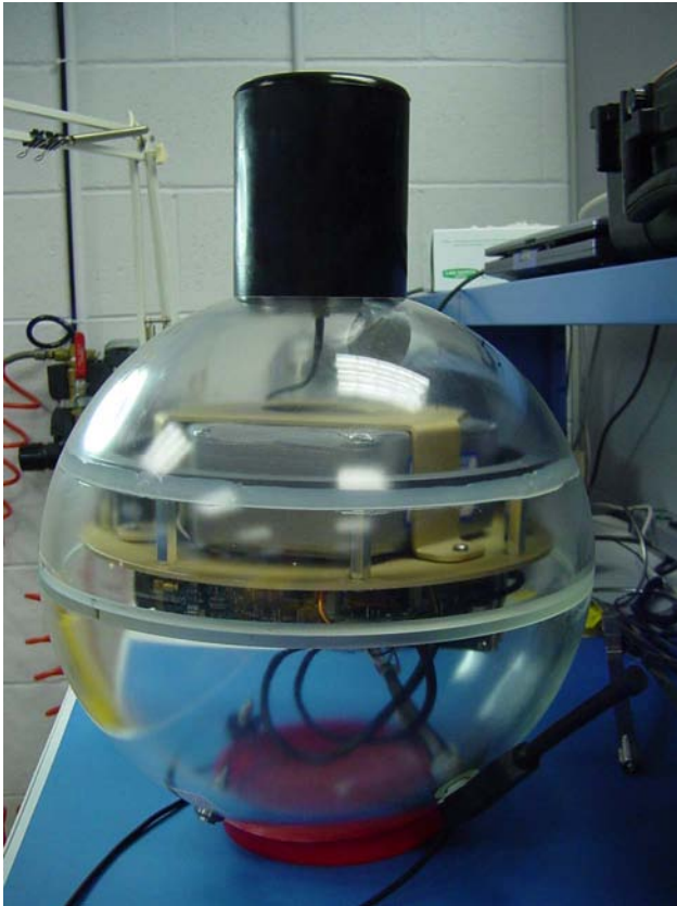
Figure 1. Teledyne Benthos' ASW Modem
