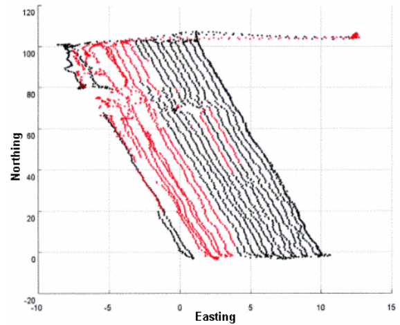
Figure 9: Check Ashtech GPS Positions
