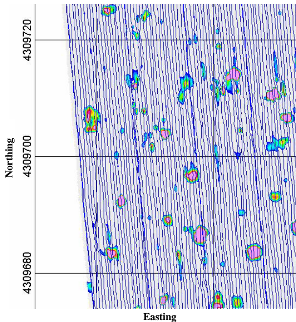
Figure 7: GPS Path For Grid 2
