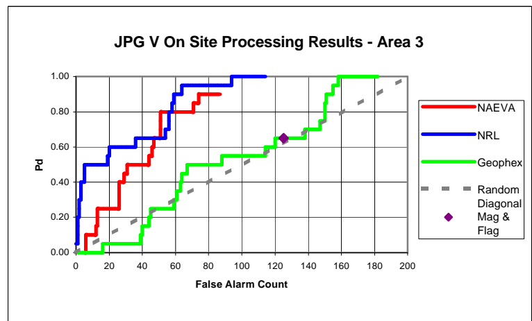
Figure 16: Composite ROC Curves
