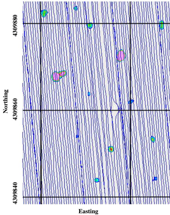
Figure 5: GPS Path For Grid 3
