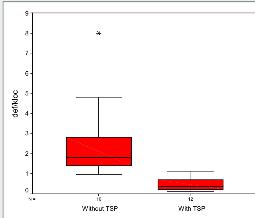
System test defect density
