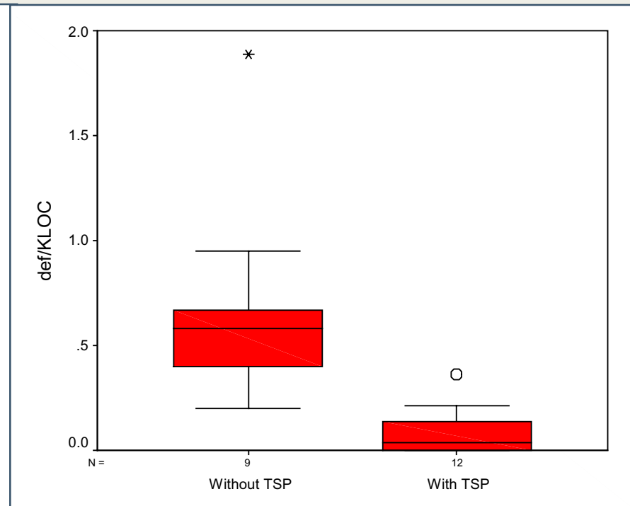
Acceptance test defect density
