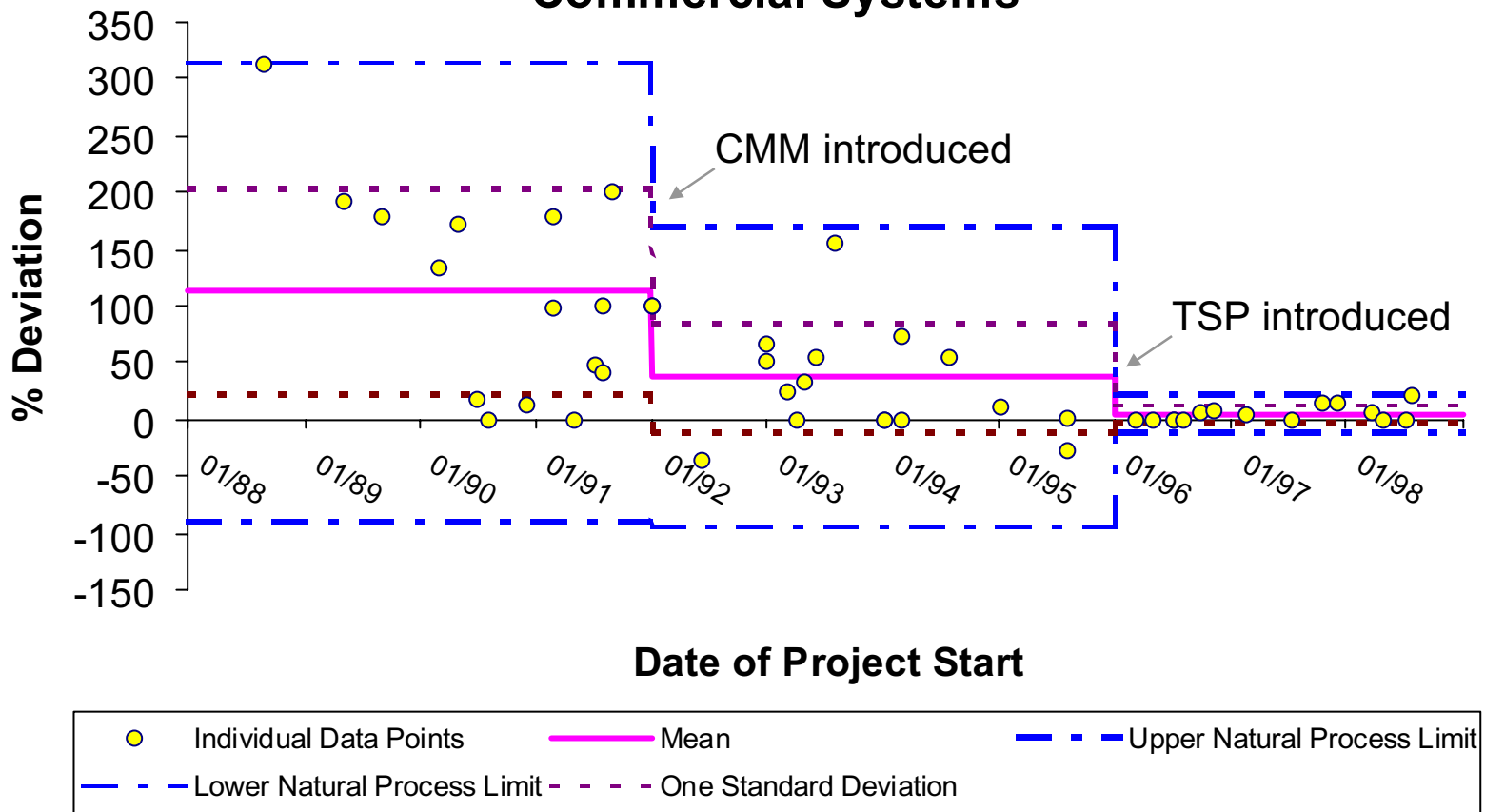
Schedule Deviation Individual Value Control Chart - Commercial Systems
