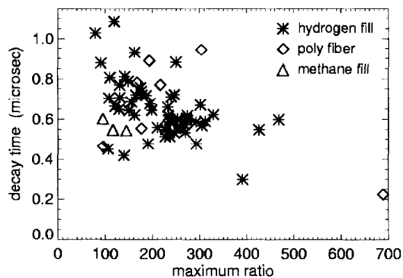
Figure 7. The hot plasma decay time as defined by the time for the ratio of open to visible-only diode signal to drop from the maximum value to 5% of the maximum value as a function of the maximum ratio for the same discharges as shown in Figs. 5 and 6.
