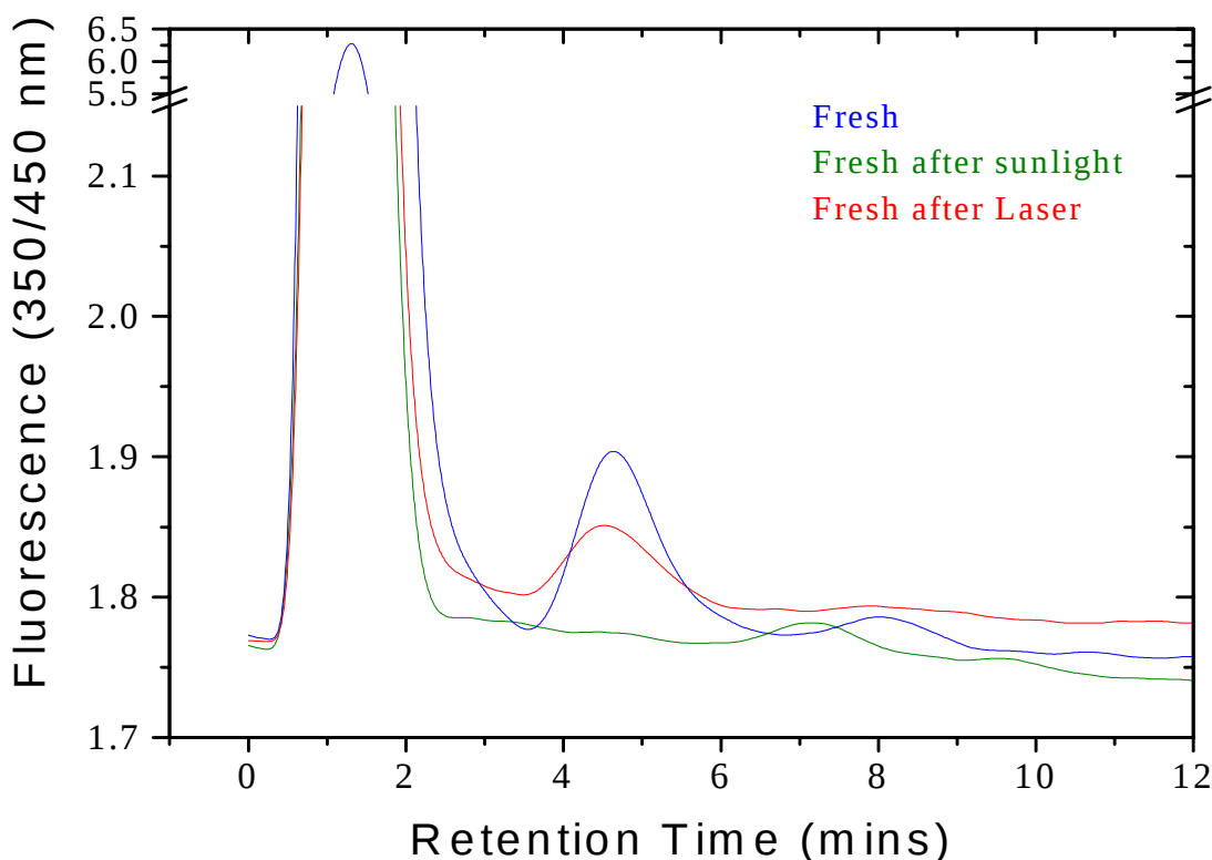
Figure 1. Fluorescence vs. retention time for irradiated South Florida water samples (3000 Dalton regenerated cellulose membrane; 0.5 \mu m filtered carrier flow: 0.1% (v/v) FL-70/0.0046M NaN 3 / ODW; flow rates: 0.3 mL/min sample inlet/outlet, 2.0 mL/min frit inlet/outlet, 1.0 mL/min crossflow)
