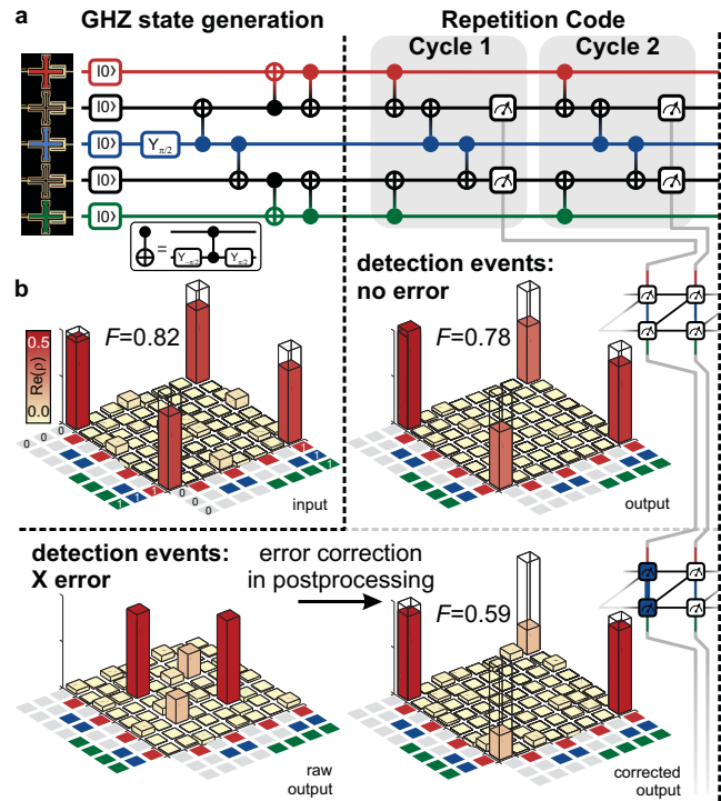
FIG. 3: Protecting the GHZ state from bit-flip errors. (a) Quantum circuit for generating the GHZ state and two cycles of the repetition code. CNOT gates are physically implemented with controlled-phase (CZ) and single qubit gates. (b) Quantum state tomography on the input, and after the repetition code conditional on the detection events: We input a GHZ state with a fidelity of 82%, and find, for the case of no detection events, a 78% fidelity GHZ state. For the detection event connecting both measure qubits, indicating a likely bit-flip error on the central data qubit, we find that through correcting in postprocessing by exchanging matrix elements we recover the major elements of the diagonal. We also recover nonzero off-diagonal elements, indicating some bit-flip errors are coherent.
