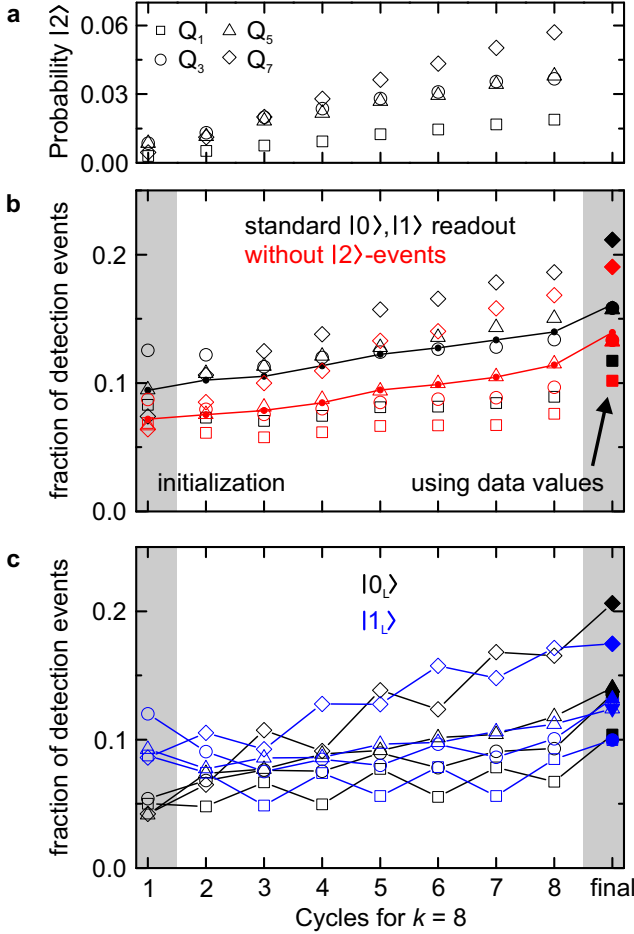
FIG. S17. State leakage and fraction of detection events for k=8 . (a) State leakage, |2\rangle -state population, for the four measurement qubits. Note that increase in measured |2\rangle state population can come from misidentification of increasing |1\rangle state population. (b) Fraction of detection events for the four measure qubits as a function of cycle number for standard |0\rangle and |1\rangle state discrimination (black), and without |2\rangle -events. Solid lines denote the averages. (c) Fraction of detection events for data qubit input states |00000\rangle and |11111\rangle , showing a clear alternating pattern of increased detection events when measure qubits are likely in the |1\rangle state. Used data is without |2\rangle -events.
