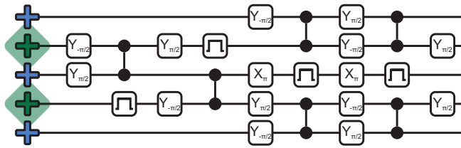
FIG. S31. Quantum circuit for the generation of the GHZ state. Rectangular gates indicate detuning pulses.
