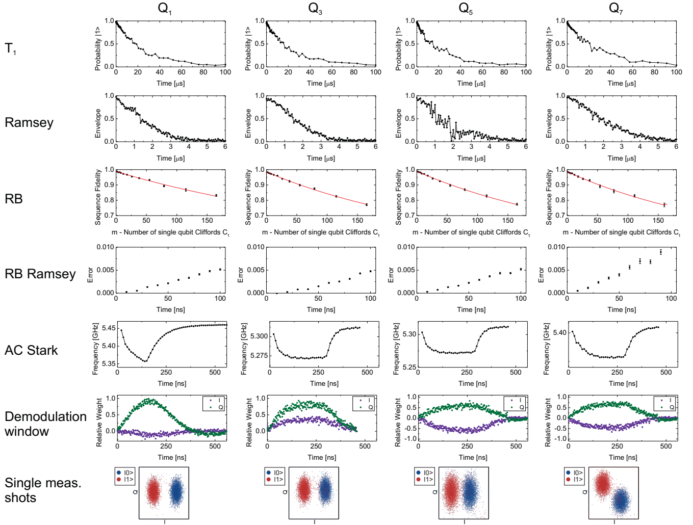
FIG. S23. Measure qubit characterization. We measure coherence, gate and readout properties on the four measure qubits. We find T_1 values in the 20-30 \mu\text{s} range for these operating points. Ramsey 1/e decay times are in the 2-3 \mu\text{s} range. Single qubit gate fidelities all meet or exceed 0.999. The RB Ramsey 12 experiment shows that the Ramsey 1/e time is not a limitation to gate fidelity. The AC stark shift and optimal demodulation windows displayed are used to achieve separation fidelities > 0.998 .
