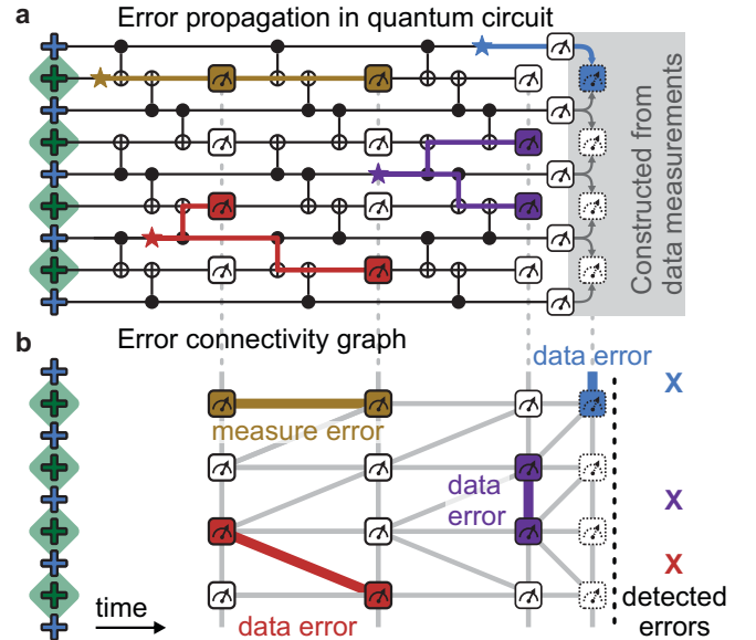
FIG. 2: Error propagation and identification. (a) The quantum circuit for three cycles of the repetition code, and examples of errors. Errors propagate horizontally in time, and vertically through entangling gates. Different errors lead to different detection patterns: An error on a measure qubit (gold) is detected in two subsequent rounds. Data qubit errors (purple, red, blue) are detected on neighbouring measurement qubits in the same or next cycle. Data errors after the last round (blue) are detected by constructing the final set of \hat{Z}\hat{Z} eigenvalues from the data qubit measurements. (b) The connectivity graph for the quantum circuit above, showing measurements and possible patterns of detection events (grey), see text. The example detection events and their connections are highlighted, the corresponding detected errors are shown on the right, which when applied, will recover the input data qubit state.
