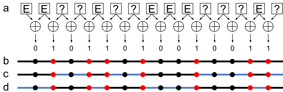
FIG. S2. Processing perfect parity measurements, large example. (a) 15 initially identical copies of an unknown bit suffer errors at unknown locations leading to a specific pattern of pairwise parity measurements. (b) Graph problem corresponding to the parity measurements. Our goal is to connect the colored vertices in pairs or to a graph boundary using the minimum total number of edges. (c) Non-optimal weight 8 graph solution. (d) Optimal weight 7 graph solution, i.e. contains the fewest errors. Note that after applying corrections corresponding to the blue edges, we will restore the data to its original state using the optimal graph solution, and the bit-inverse of the original state using the non-optimal graph solution. This is a generic property — after correction one will always obtain the original data or its perfect bit-inverse.
