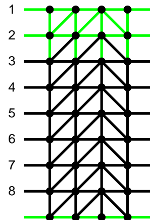
FIG. S13. Green edges denote geometrically- or weight-distinct edges. Every black edge is equivalent to a green edge by time translation. The relatively low number of unique edges is due to the cyclic nature of the repetition code, and hence the cyclic nature of error propagation. Two edges for coping with leakage are also optimized, but not shown as they are dynamically added when leakage is detected.
