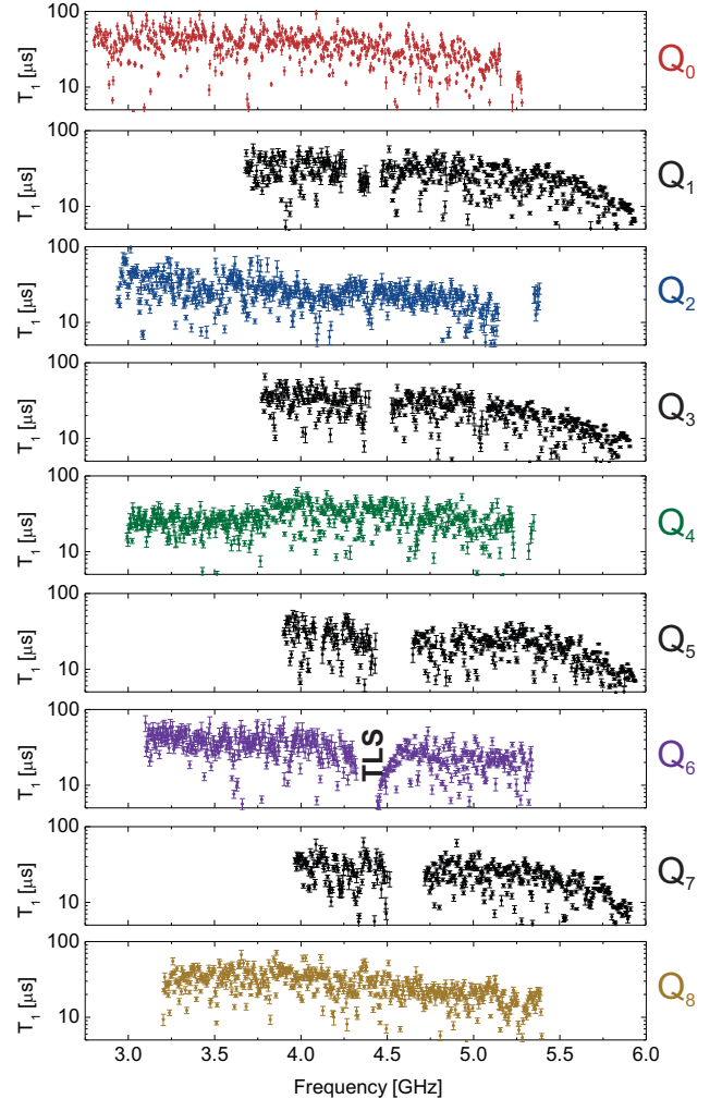
FIG. S18. Energy Relaxation. T_1 for all nine qubits as a function of frequency. Xmon qubits have a 24\ \mu\text{m} gap and 24\ \mu\text{m} center width for the capacitor. Missing data due to coherent swapping with other qubits or low quality fits. Two-level state (TLS) seen in the spectrum of Q_6 .
