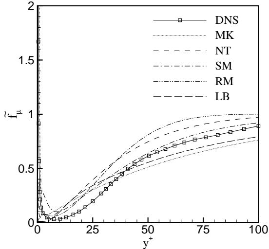
Figure 3. Comparison of model damping functions against \tilde{f}_\mu computed from DNS data of a Mach 4 boundary layer. The model codes are given in Table 1.
