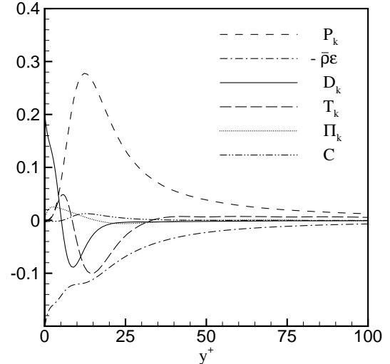
Figure 4. Budget of k -equation using DNS data of a Mach 4 boundary layer. The source terms are normalized by \bar{\rho}_w u_\tau^4 / \bar{\nu}_w .
