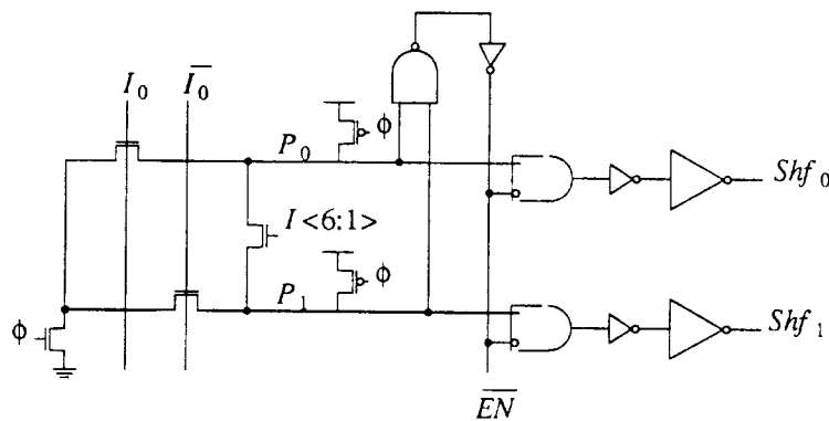
Figure 4.19. Transition detector for enabling the shifter. When the decoder precharges, both P0 and P1 are high. Only one out of P0 or P1 can be low after the shifter decoder has evaluat-
