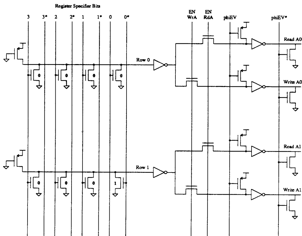
Figure 4.6. The Register File Decoder. Two sets of decoders are necessary to read and write both busses. The design is pseudo-static, with pullup by P channel transistors with gates tied to ground.
