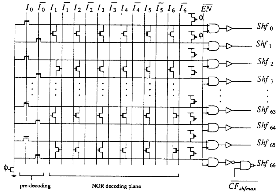
Figure 4.18. The shifter decode matrix. Bit<0> is pre-decoded, eliminating the need for Ground lines and reducing the number of pass gates in the decoder matrix by almost 50%.
