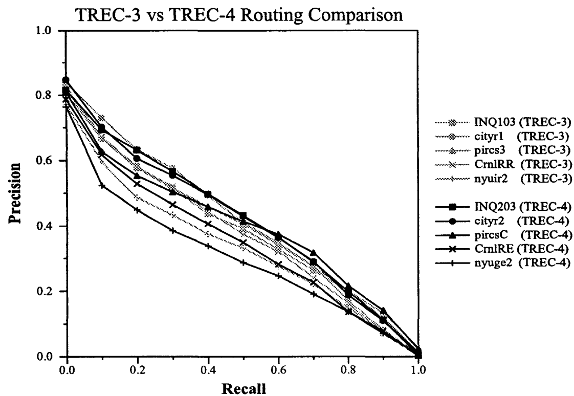
Figure 13. Comparison of Routing Results for TREC-3 and TREC-4
