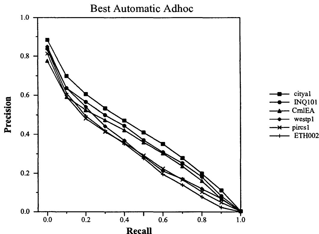
Figure 3. Best TREC-3 Automatic Adhoc Results.
