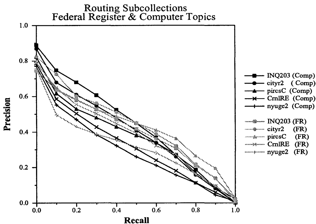
Figure 12. Comparison of Results for Federal Register Topics and Computer Topics
