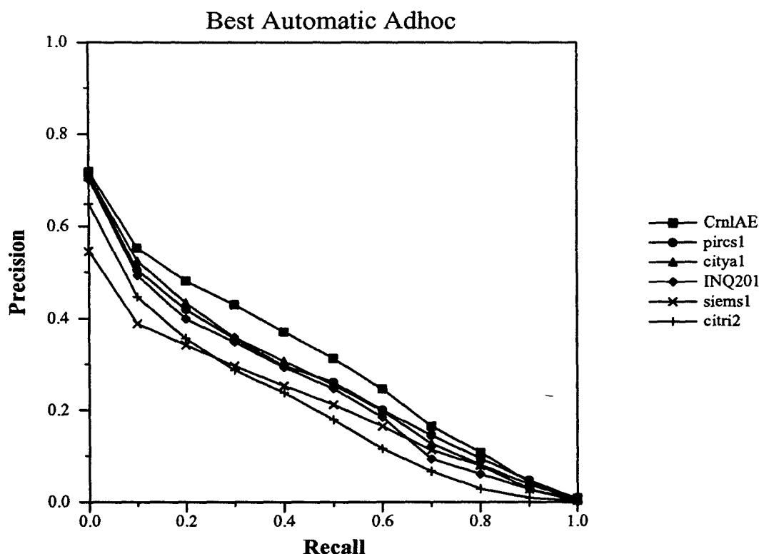
Figure 6. Best TREC-4 Automatic Adhoc Results.
