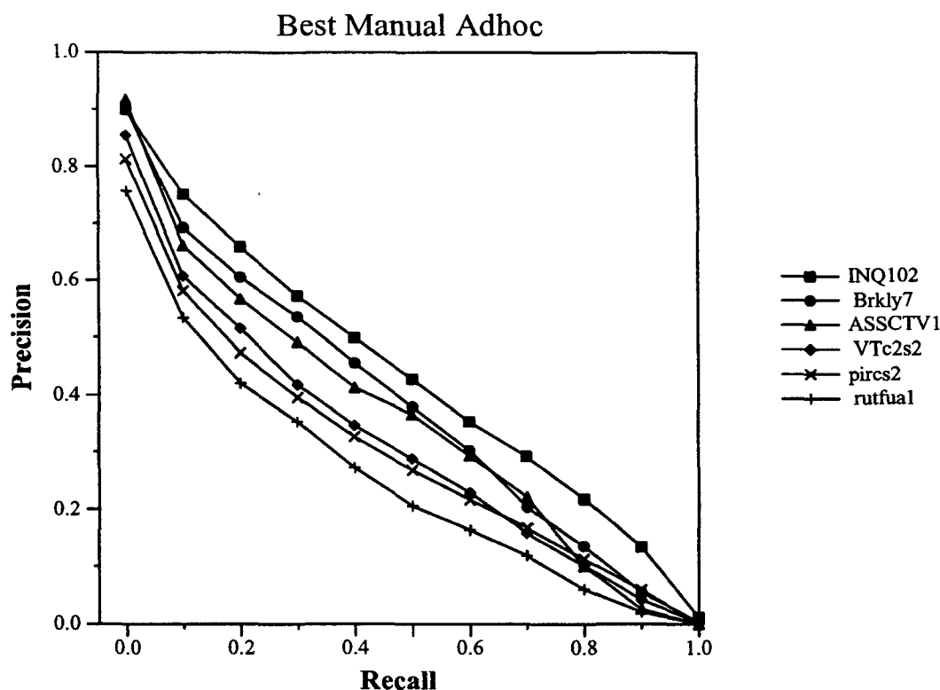
Figure 4. Best TREC-3 Manual Adhoc Results.
