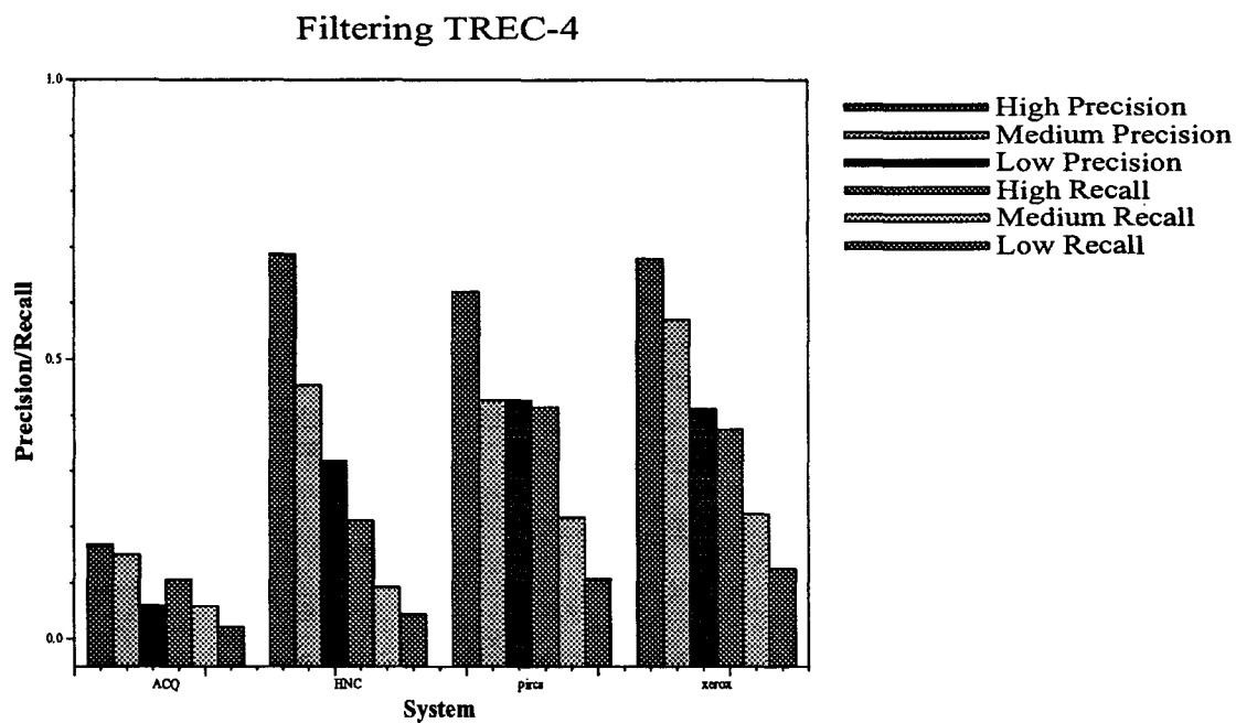
Figure 17. Results of TREC-4 Filtering Track
