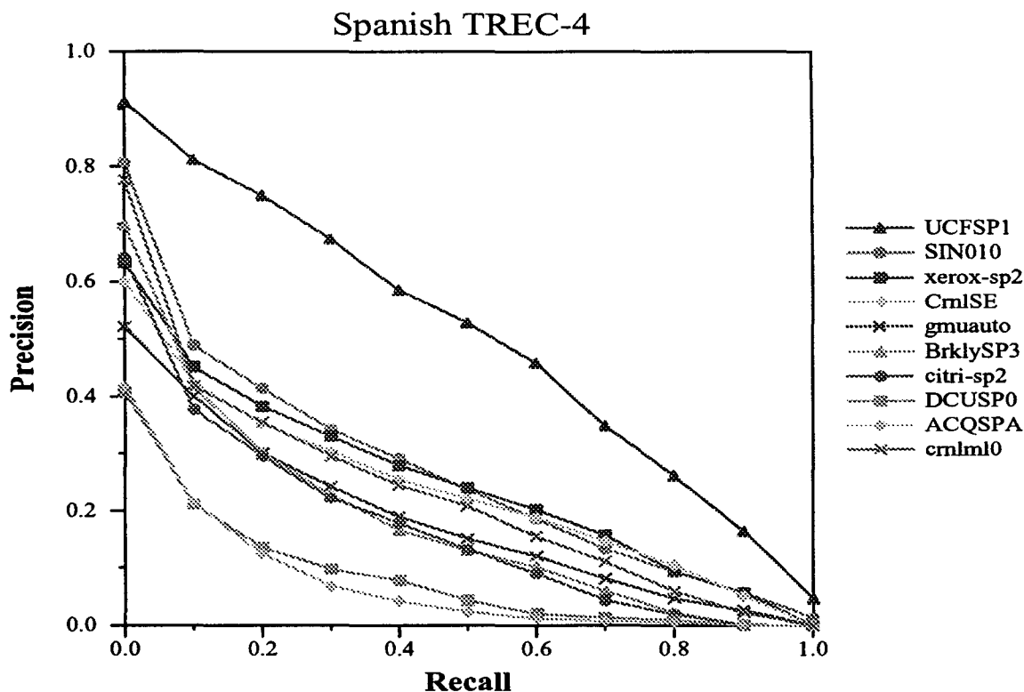
Figure 14. Results of TREC-4 Spanish Track
