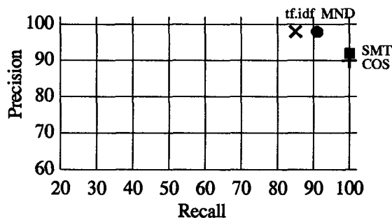
Figure 6.2-3. Set 3 Classification Results
