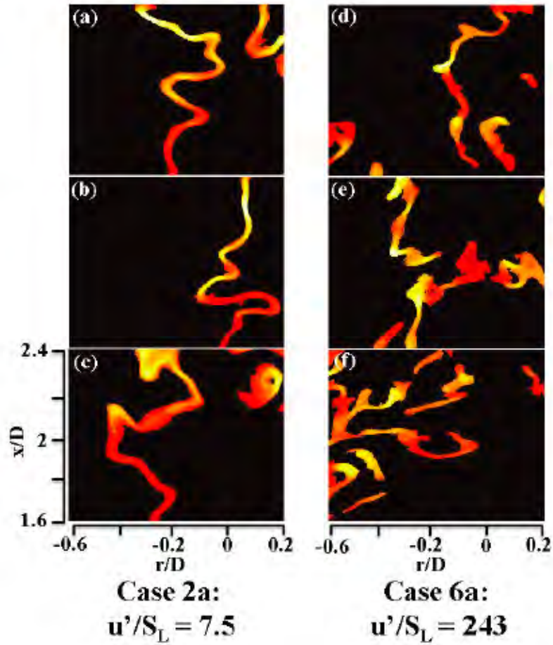
Figure 10. Reaction zones instantaneous images at random times for Case 2a and Case 6a.
