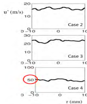
Figure 5. Turbulence level profiles at Hi-Pilot burner exit.
