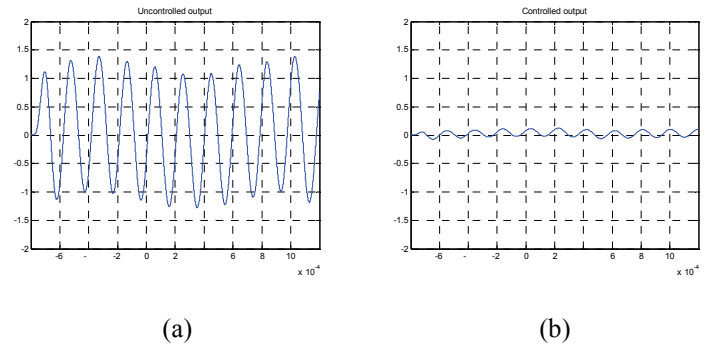
Figure 6. Experimental result of rebalance loop control
