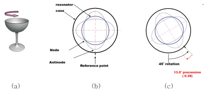
Figure 1. Operating principle of HRG
