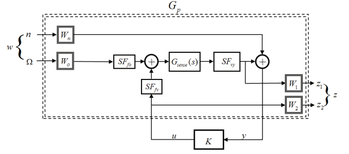
Figure 3. Two port system of HRG.
