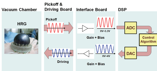
Figure 4. Configuration of rebalance loop test
