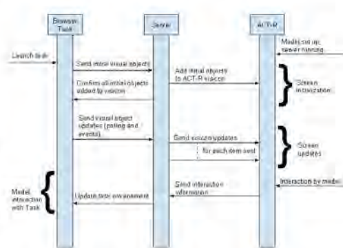
Figure 2: Information flow through SIMCog-JS. The information events start with the modeler initiating the Java ACT-R model and then launching the browser-based task. SIMCog-JS then connects the two environments. The vertical dimension captures time flowing from top to bottom.
