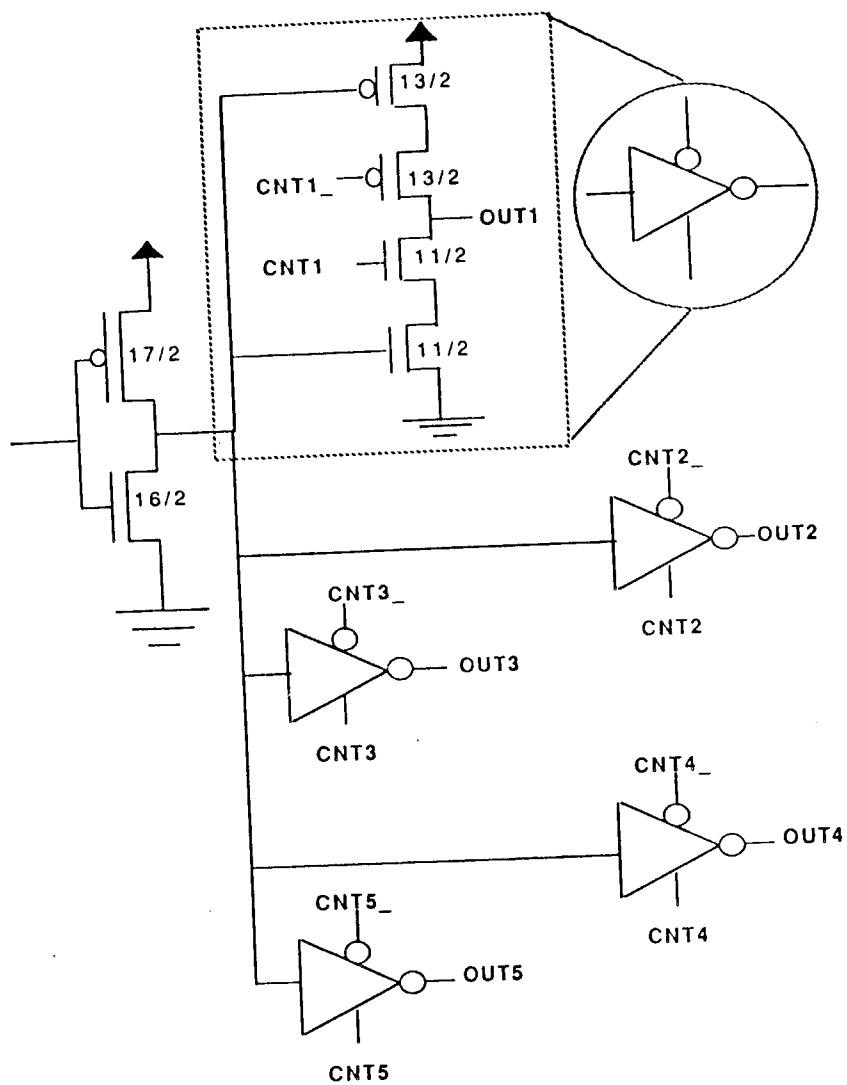
5 OUTPUTS TRI-STATE BUFFER
